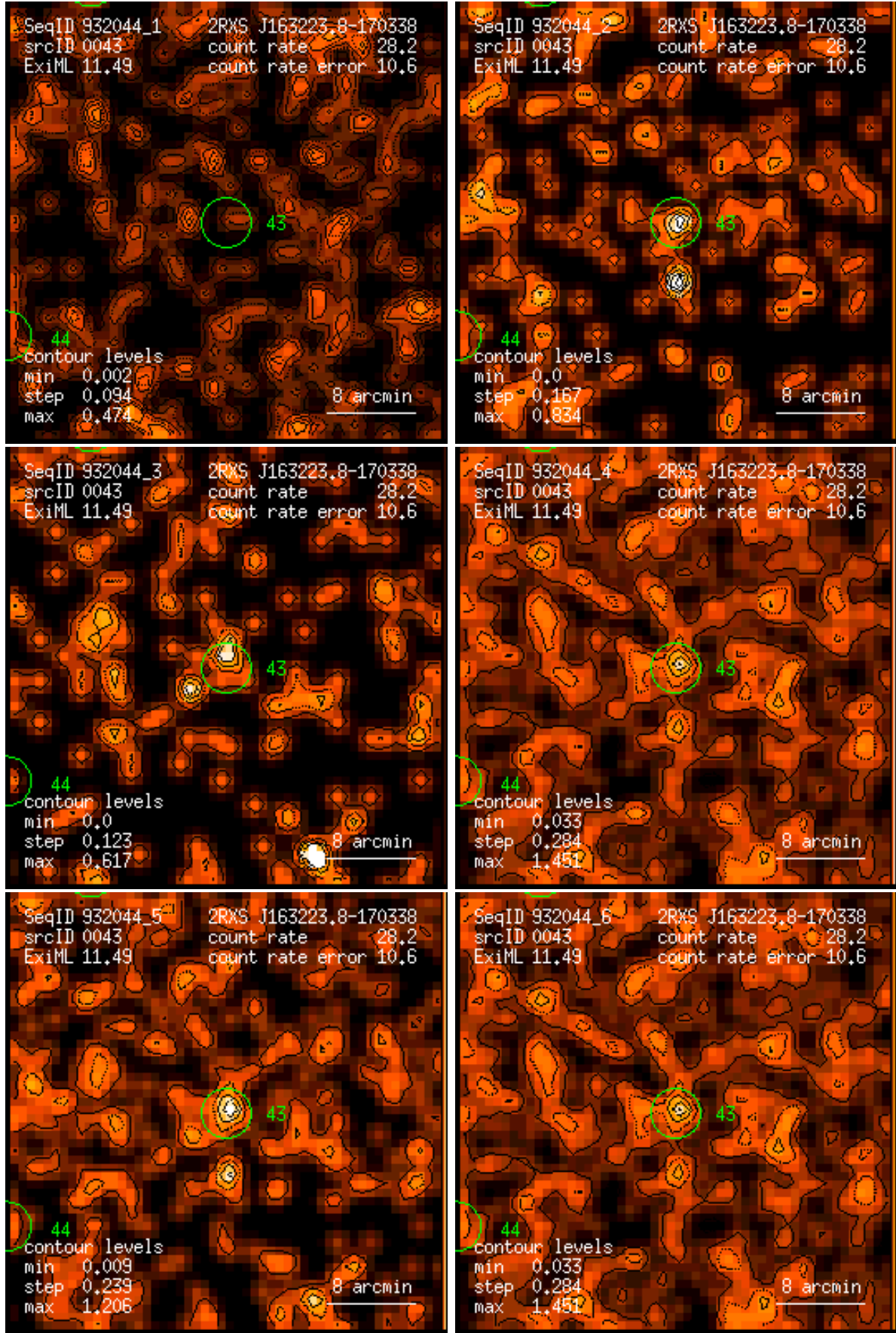
Figure 43: RASS 932044: detection 0043: band rate images, Gaussian filter: (1) PSPC channels 11 – 41, (2) 52 – 90, (3) 91 – 201, (4) 11 – 235, (5) 52 – 201, (6) 11 – 201. Broad band rates in counts/ks. Band rate contour levels in counts/ks/arcmin 2 .
