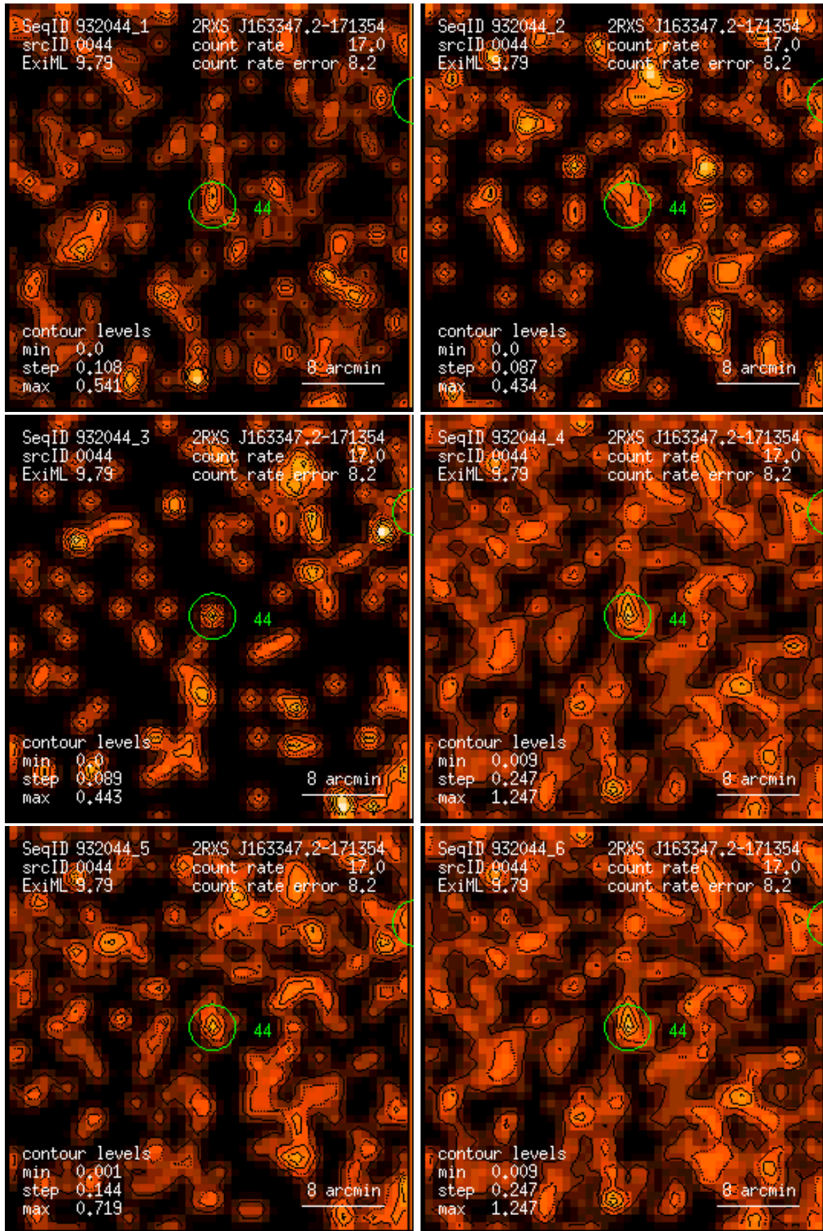
Figure 44: RASS 932044: detection 0044: band rate images, Gaussian filter: (1) PSPC channels 11 – 41, (2) 52 – 90, (3) 91 – 201, (4) 11 – 235, (5) 52 – 201, (6) 11 – 201. Broad band rates in counts/ks. Band rate contour levels in counts/ks/arcmin 2 .
