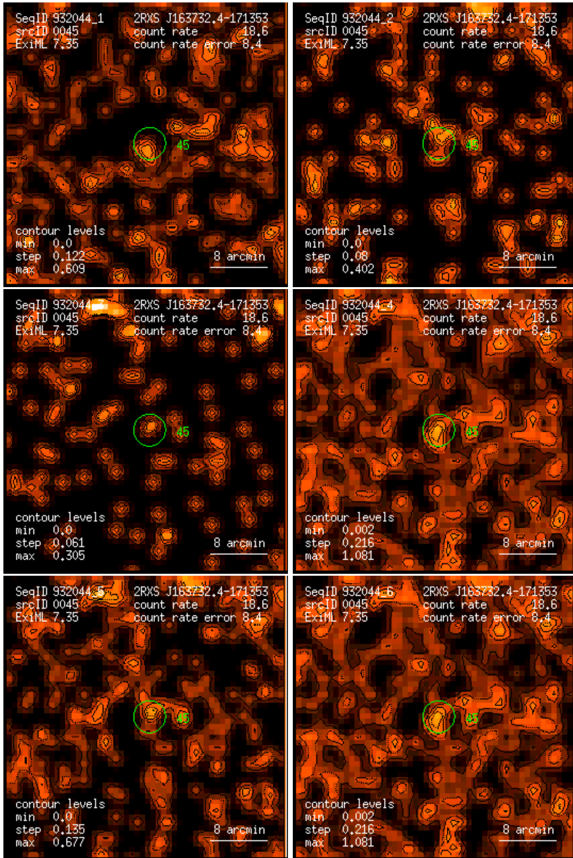
Figure 45: RASS 932044: detection 0045: band rate images, Gaussian filter: (1) PSPC channels 11 – 41, (2) 52 – 90, (3) 91 – 201, (4) 11 – 235, (5) 52 – 201, (6) 11 – 201. Broad band rates in counts/ks. Band rate contour levels in counts/ks/arcmin 2 .
