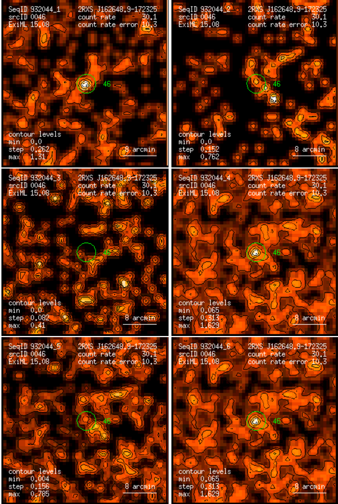
Figure 46: RASS 932044: detection 0046: band rate images, Gaussian filter: (1) PSPC channels 11 – 41, (2) 52 – 90, (3) 91 – 201, (4) 11 – 235, (5) 52 – 201, (6) 11 – 201. Broad band rates in counts/ks. Band rate contour levels in counts/ks/arcmin 2 .
