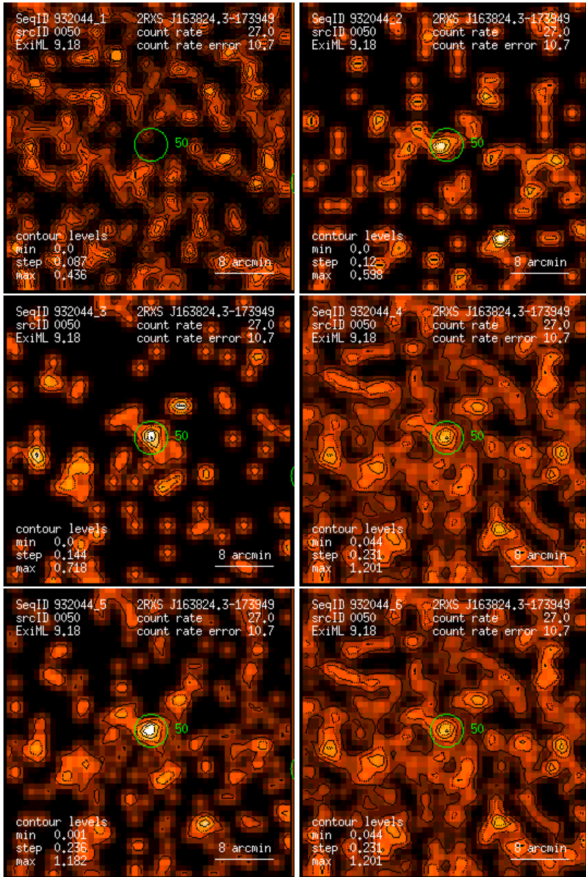
Figure 50: RASS 932044: detection 0050: band rate images, Gaussian filter: (1) PSPC channels 11 – 41, (2) 52 – 90, (3) 91 – 201, (4) 11 – 235, (5) 52 – 201, (6) 11 – 201. Broad band rates in counts/ks. Band rate contour levels in counts/ks/arcmin 2 .
