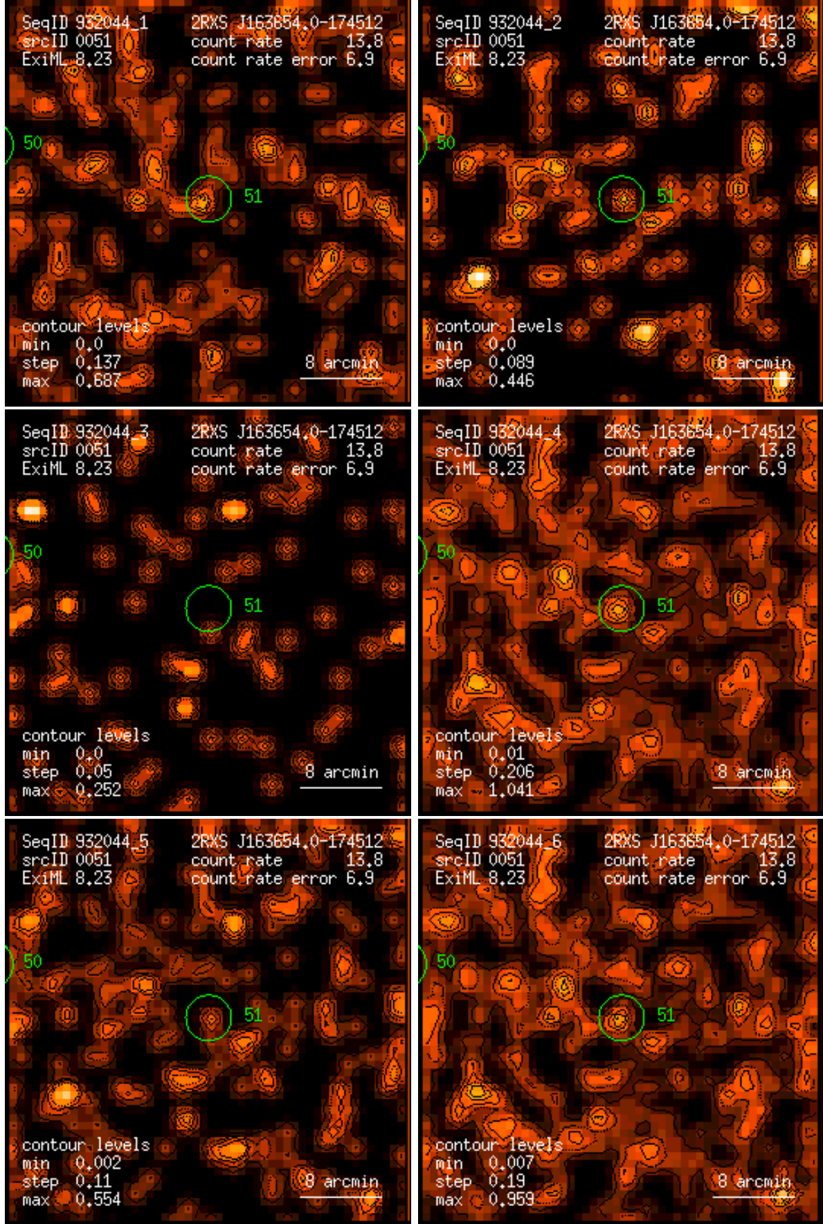
Figure 51: RASS 932044: detection 0051: band rate images, Gaussian filter: (1) PSPC channels 11 – 41, (2) 52 – 90, (3) 91 – 201, (4) 11 – 235, (5) 52 – 201, (6) 11 – 201. Broad band rates in counts/ks. Band rate contour levels in counts/ks/arcmin 2 .
