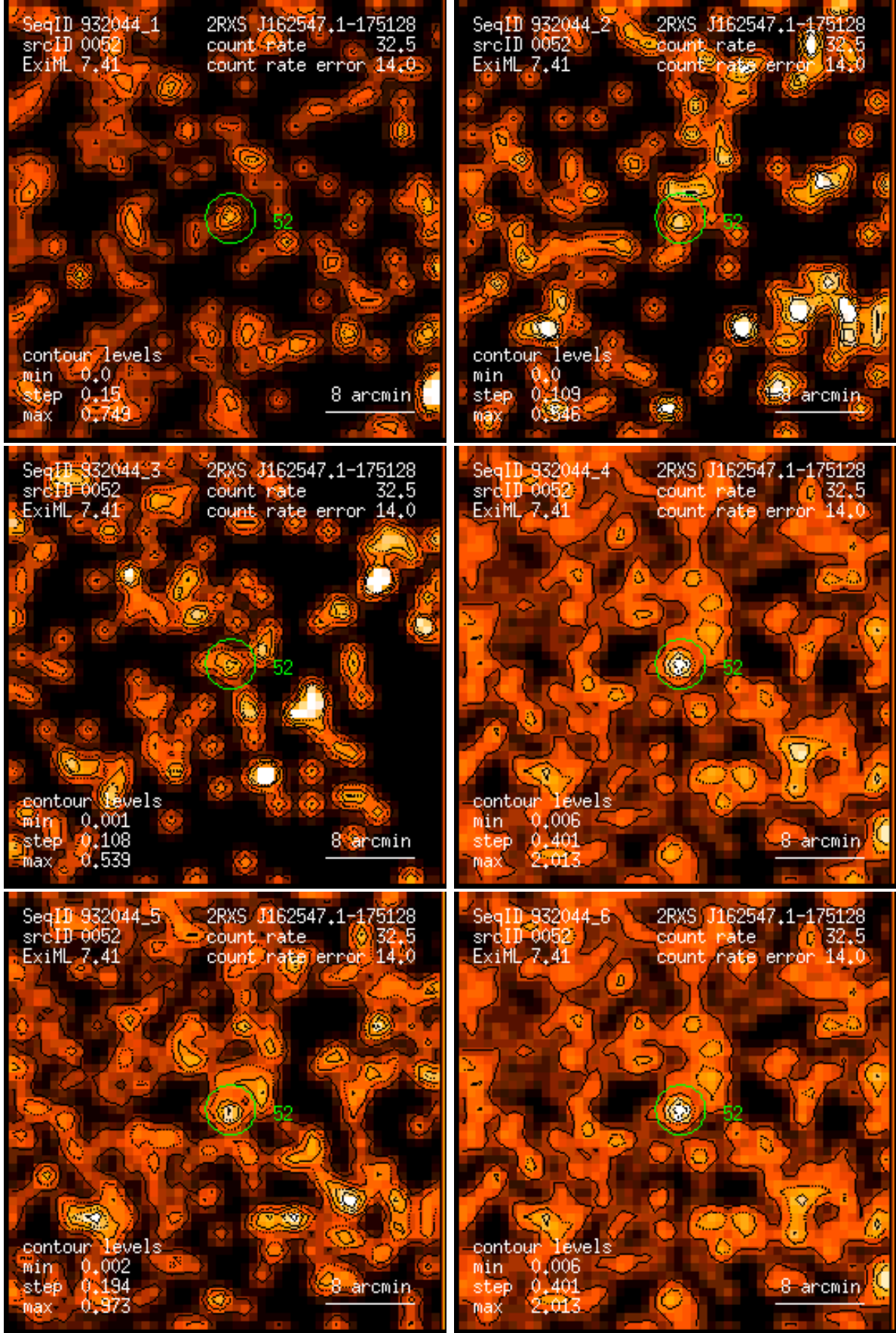
Figure 52: RASS 932044: detection 0052: band rate images, Gaussian filter: (1) PSPC channels 11 – 41, (2) 52 – 90, (3) 91 – 201, (4) 11 – 235, (5) 52 – 201, (6) 11 – 201. Broad band rates in counts/ks. Band rate contour levels in counts/ks/arcmin 2 .
