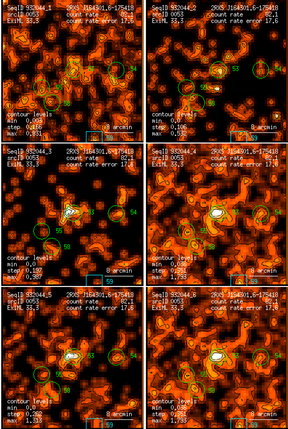
Figure 53: RASS 932044: detection 0053: band rate images, Gaussian filter: (1) PSPC channels 11 – 41, (2) 52 – 90, (3) 91 – 201, (4) 11 – 235, (5) 52 – 201, (6) 11 – 201. Broad band rates in counts/ks. Band rate contour levels in counts/ks/arcmin 2 .
