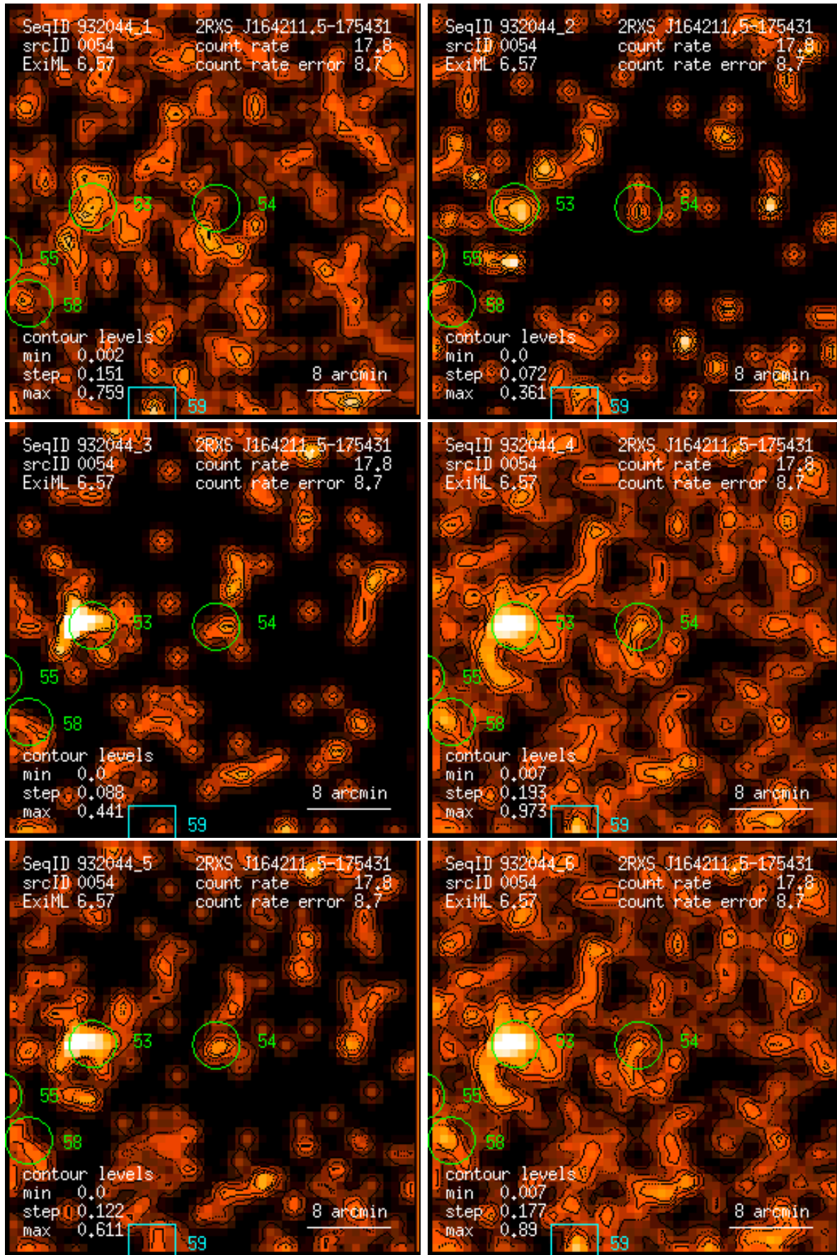
Figure 54: RASS 932044: detection 0054: band rate images, Gaussian filter: (1) PSPC channels 11 – 41, (2) 52 – 90, (3) 91 – 201, (4) 11 – 235, (5) 52 – 201, (6) 11 – 201. Broad band rates in counts/ks. Band rate contour levels in counts/ks/arcmin 2 .
