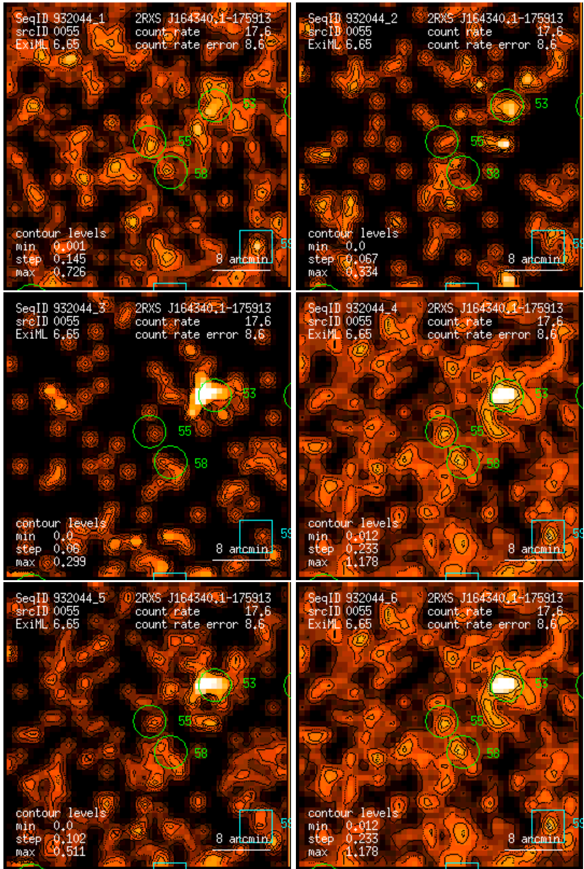
Figure 55: RASS 932044: detection 0055: band rate images, Gaussian filter: (1) PSPC channels 11 – 41, (2) 52 – 90, (3) 91 – 201, (4) 11 – 235, (5) 52 – 201, (6) 11 – 201. Broad band rates in counts/ks. Band rate contour levels in counts/ks/arcmin 2 .
