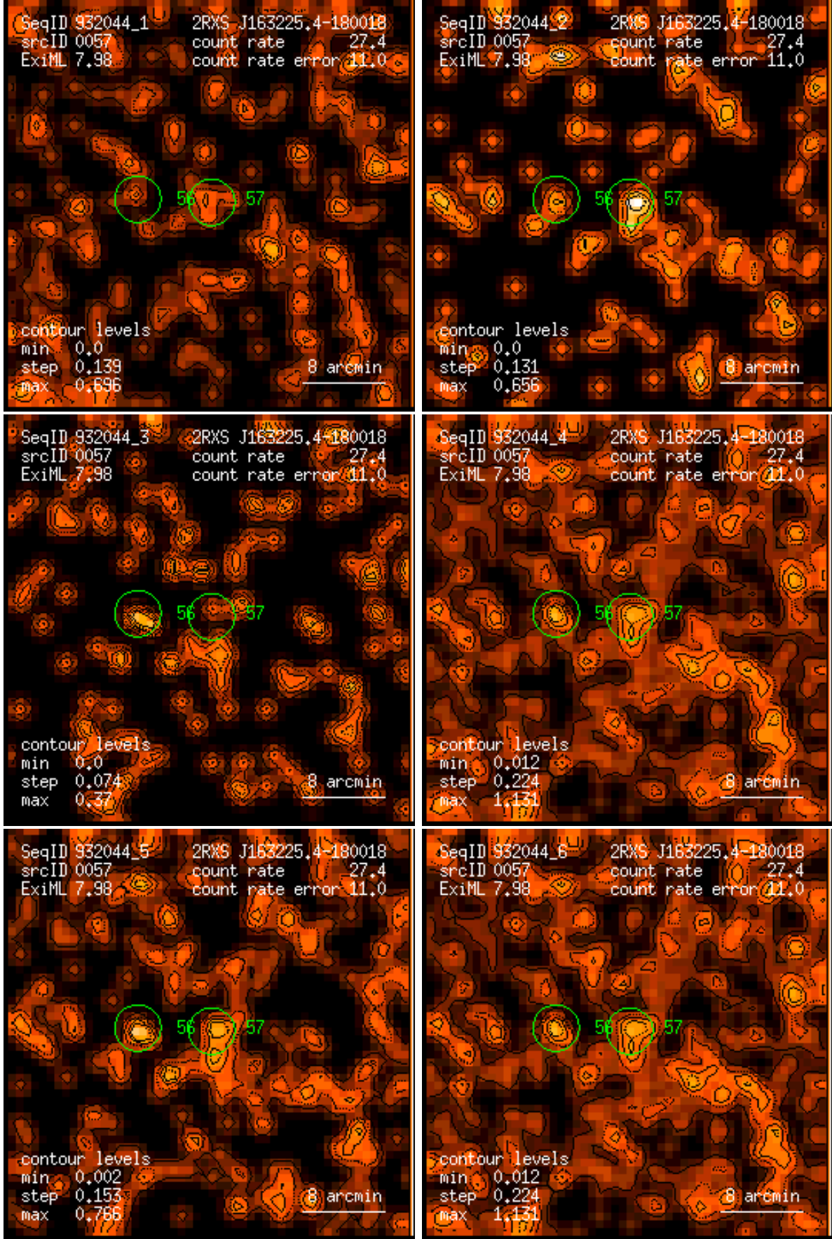
Figure 57: RASS 932044: detection 0057: band rate images, Gaussian filter: (1) PSPC channels 11 – 41, (2) 52 – 90, (3) 91 – 201, (4) 11 – 235, (5) 52 – 201, (6) 11 – 201. Broad band rates in counts/ks. Band rate contour levels in counts/ks/arcmin 2 .
