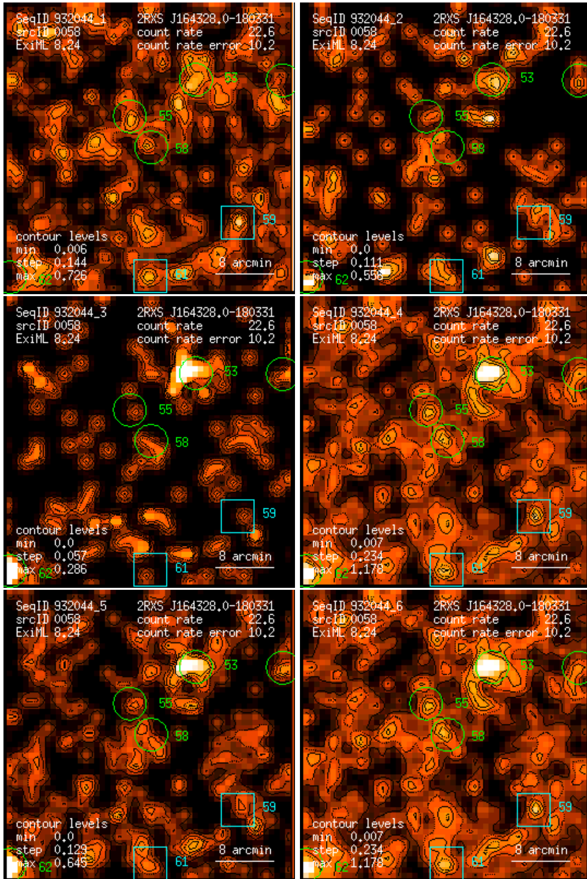
Figure 58: RASS 932044: detection 0058: band rate images, Gaussian filter: (1) PSPC channels 11 – 41, (2) 52 – 90, (3) 91 – 201, (4) 11 – 235, (5) 52 – 201, (6) 11 – 201. Broad band rates in counts/ks. Band rate contour levels in counts/ks/arcmin 2 .
