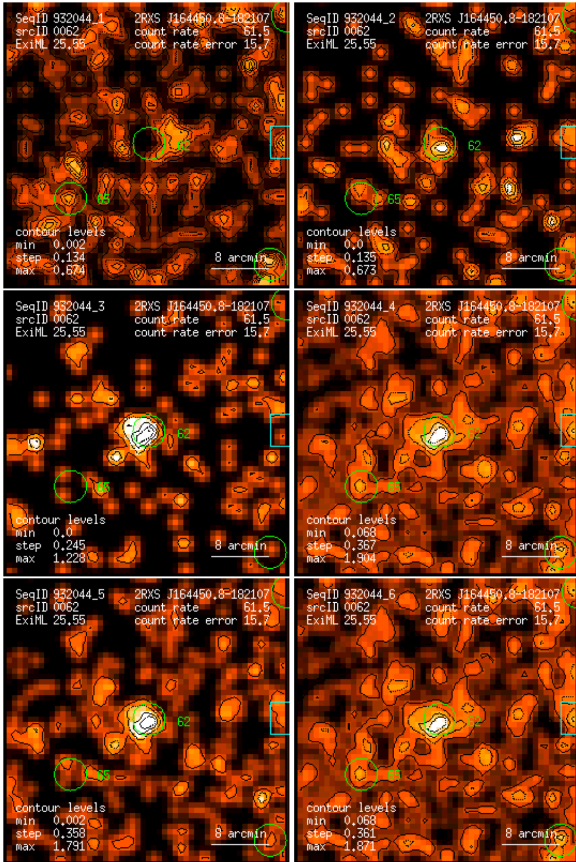
Figure 62: RASS 932044: detection 0062: band rate images, Gaussian filter: (1) PSPC channels 11 – 41, (2) 52 – 90, (3) 91 – 201, (4) 11 – 235, (5) 52 – 201, (6) 11 – 201. Broad band rates in counts/ks. Band rate contour levels in counts/ks/arcmin 2 .
