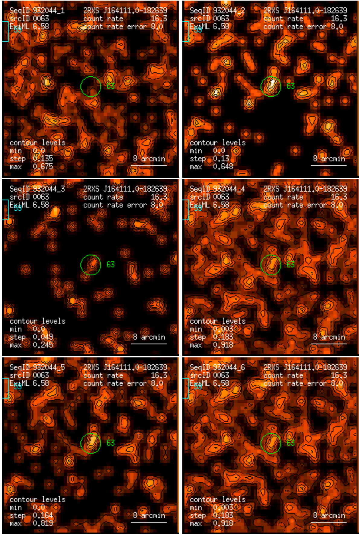
Figure 63: RASS 932044: detection 0063: band rate images, Gaussian filter: (1) PSPC channels 11 – 41, (2) 52 – 90, (3) 91 – 201, (4) 11 – 235, (5) 52 – 201, (6) 11 – 201. Broad band rates in counts/ks. Band rate contour levels in counts/ks/arcmin 2 .
