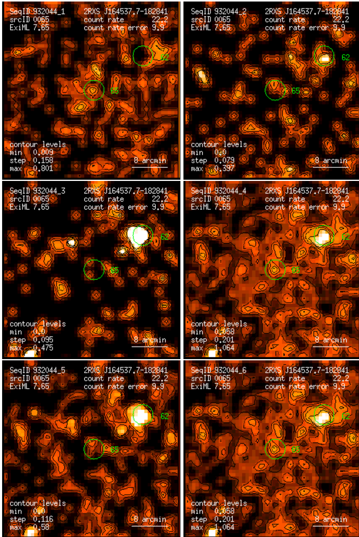
Figure 65: RASS 932044: detection 0065: band rate images, Gaussian filter: (1) PSPC channels 11 – 41, (2) 52 – 90, (3) 91 – 201, (4) 11 – 235, (5) 52 – 201, (6) 11 – 201. Broad band rates in counts/ks. Band rate contour levels in counts/ks/arcmin 2 .
