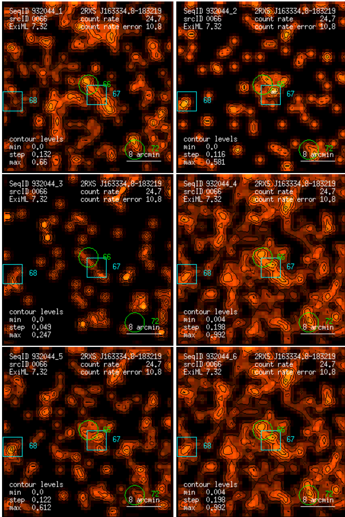
Figure 66: RASS 932044: detection 0066: band rate images, Gaussian filter: (1) PSPC channels 11 – 41, (2) 52 – 90, (3) 91 – 201, (4) 11 – 235, (5) 52 – 201, (6) 11 – 201. Broad band rates in counts/ks. Band rate contour levels in counts/ks/arcmin 2 .
