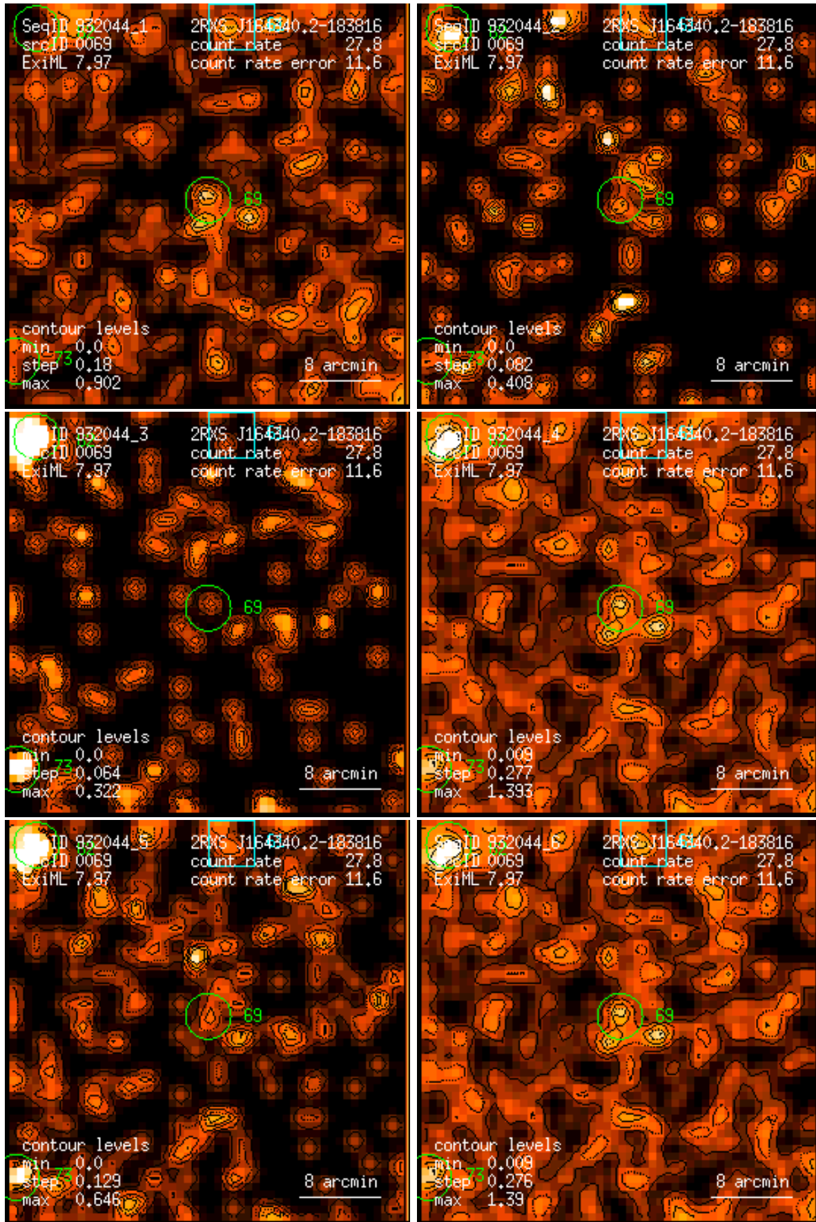
Figure 69: RASS 932044: detection 0069: band rate images, Gaussian filter: (1) PSPC channels 11 – 41, (2) 52 – 90, (3) 91 – 201, (4) 11 – 235, (5) 52 – 201, (6) 11 – 201. Broad band rates in counts/ks. Band rate contour levels in counts/ks/arcmin 2 .
