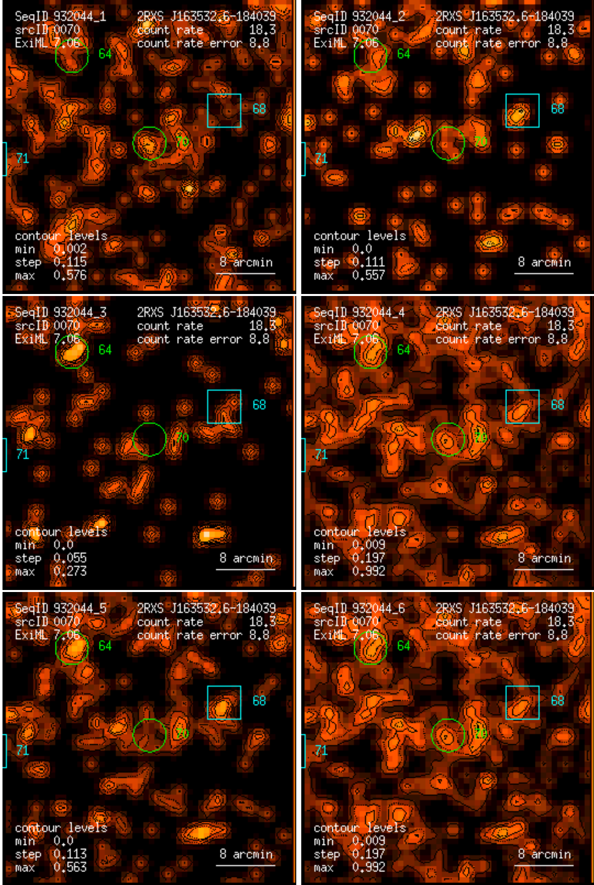
Figure 70: RASS 932044: detection 0070: band rate images, Gaussian filter: (1) PSPC channels 11 – 41, (2) 52 – 90, (3) 91 – 201, (4) 11 – 235, (5) 52 – 201, (6) 11 – 201. Broad band rates in counts/ks. Band rate contour levels in counts/ks/arcmin 2 .
