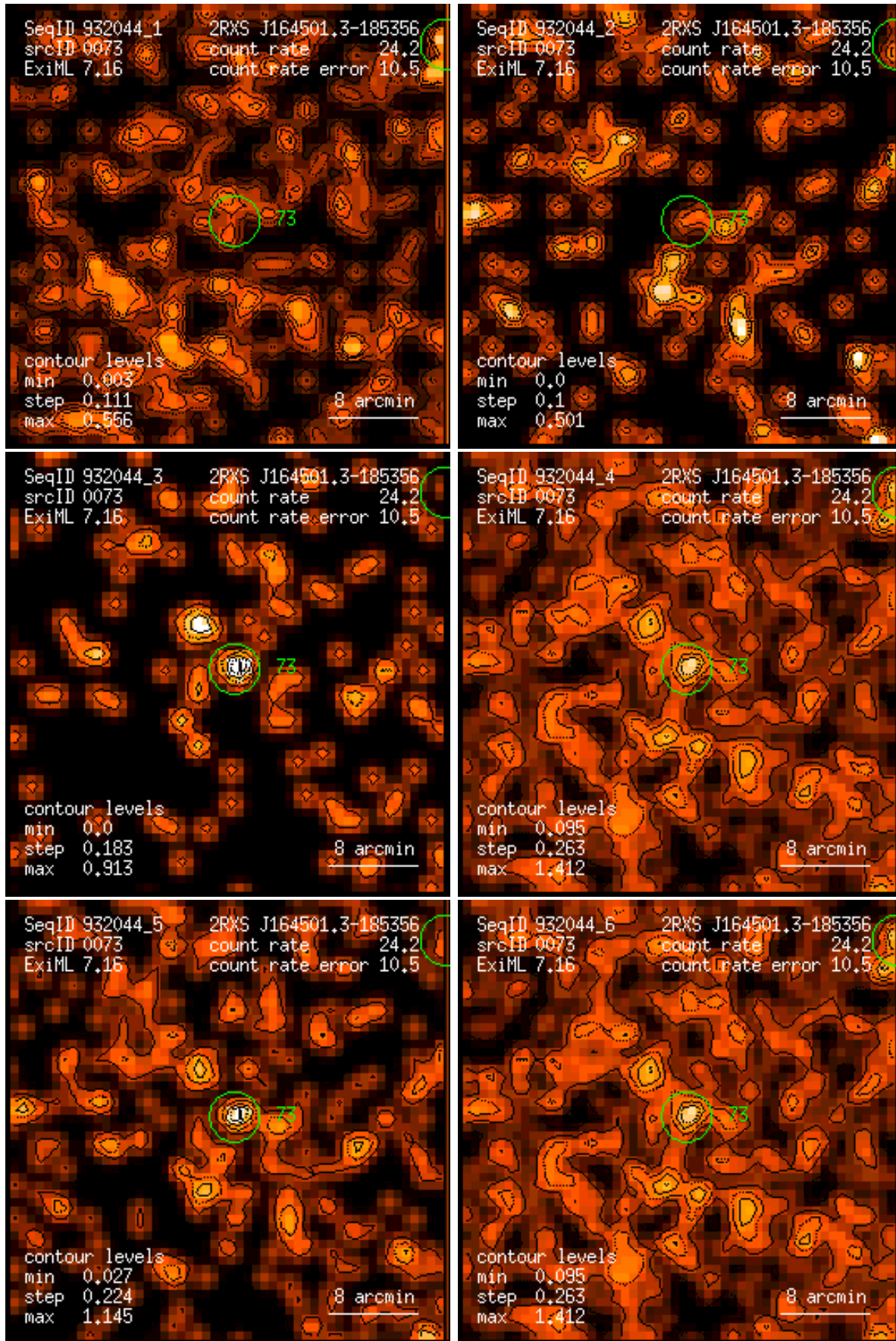
Figure 73: RASS 932044: detection 0073: band rate images, Gaussian filter: (1) PSPC channels 11 – 41, (2) 52 – 90, (3) 91 – 201, (4) 11 – 235, (5) 52 – 201, (6) 11 – 201. Broad band rates in counts/ks. Band rate contour levels in counts/ks/arcmin 2 .
