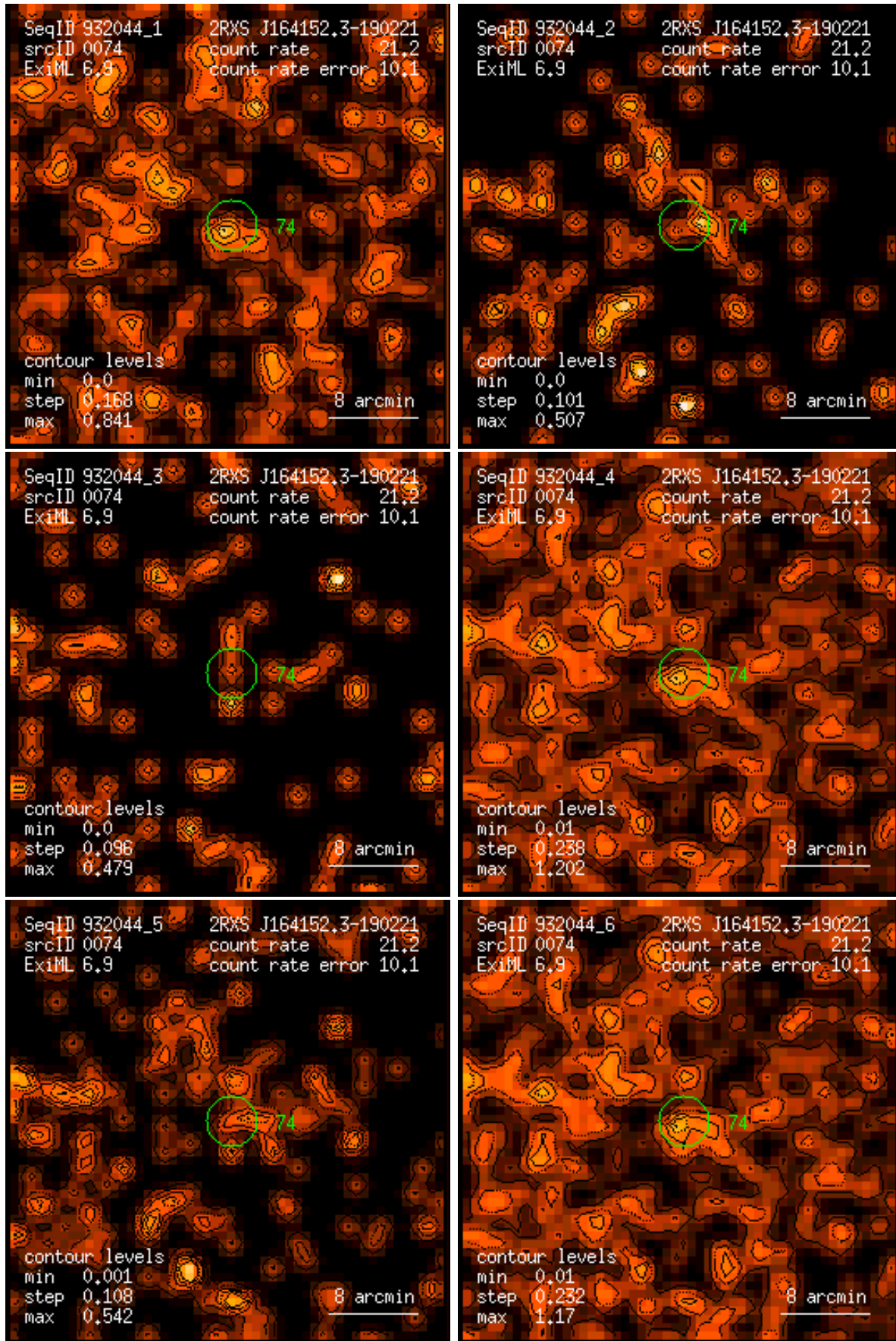
Figure 74: RASS 932044: detection 0074: band rate images, Gaussian filter: (1) PSPC channels 11 – 41, (2) 52 – 90, (3) 91 – 201, (4) 11 – 235, (5) 52 – 201, (6) 11 – 201. Broad band rates in counts/ks. Band rate contour levels in counts/ks/arcmin 2 .
