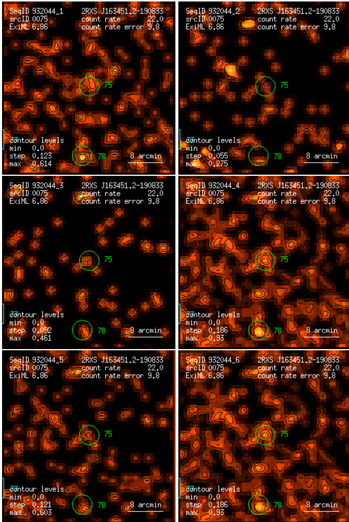
Figure 75: RASS 932044: detection 0075: band rate images, Gaussian filter: (1) PSPC channels 11 – 41, (2) 52 – 90, (3) 91 – 201, (4) 11 – 235, (5) 52 – 201, (6) 11 – 201. Broad band rates in counts/ks. Band rate contour levels in counts/ks/arcmin 2 .
