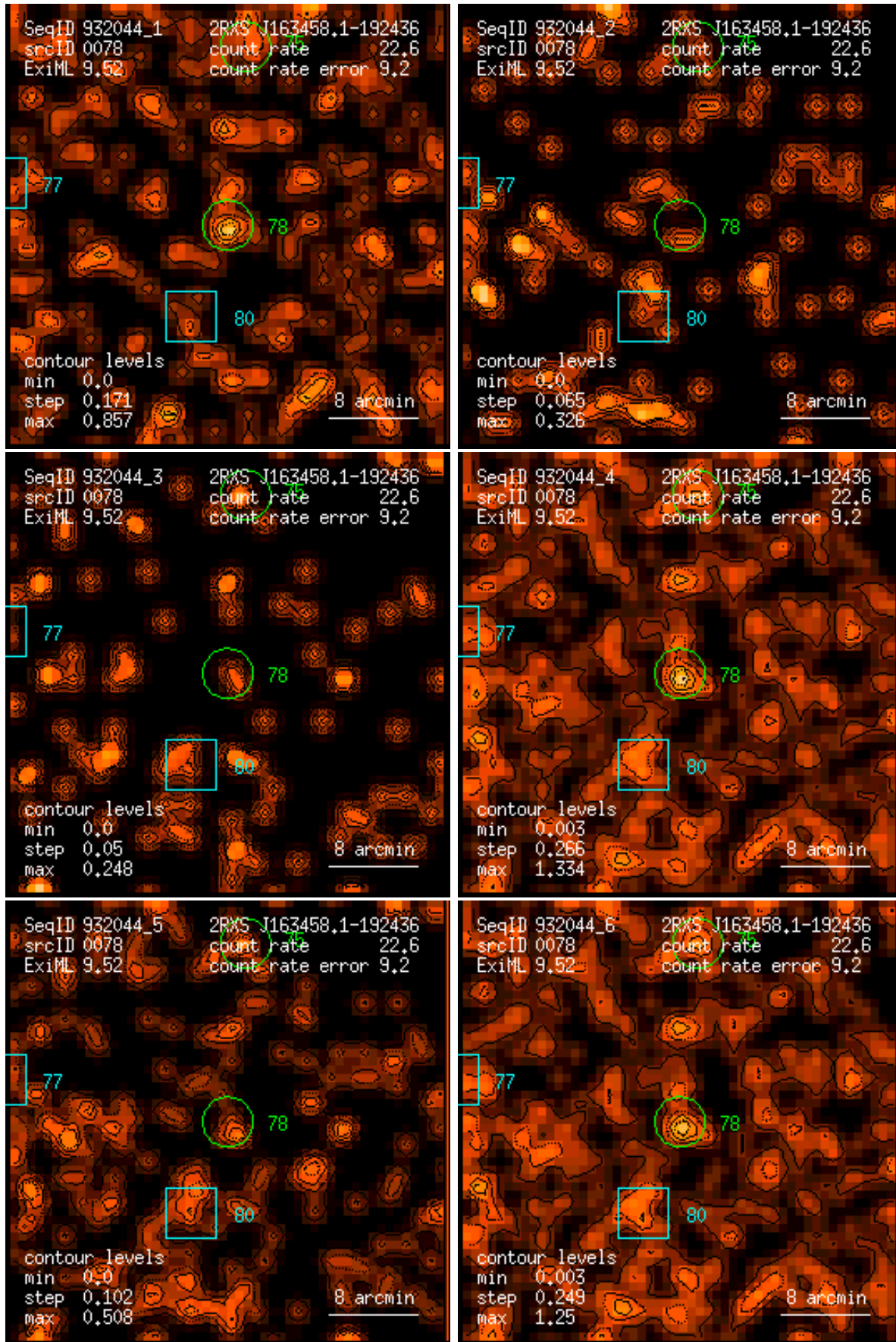
Figure 78: RASS 932044: detection 0078: band rate images, Gaussian filter: (1) PSPC channels 11 – 41, (2) 52 – 90, (3) 91 – 201, (4) 11 – 235, (5) 52 – 201, (6) 11 – 201. Broad band rates in counts/ks. Band rate contour levels in counts/ks/arcmin 2 .
