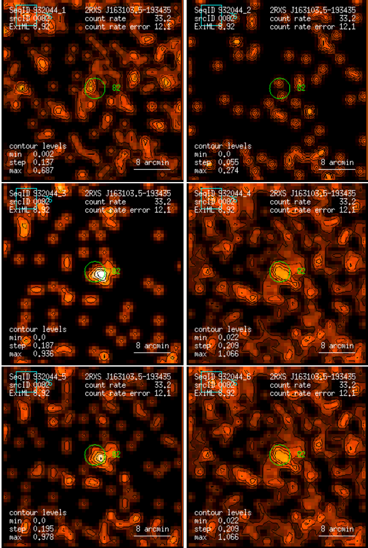
Figure 82: RASS 932044: detection 0082: band rate images, Gaussian filter: (1) PSPC channels 11 – 41, (2) 52 – 90, (3) 91 – 201, (4) 11 – 235, (5) 52 – 201, (6) 11 – 201. Broad band rates in counts/ks. Band rate contour levels in counts/ks/arcmin 2 .
