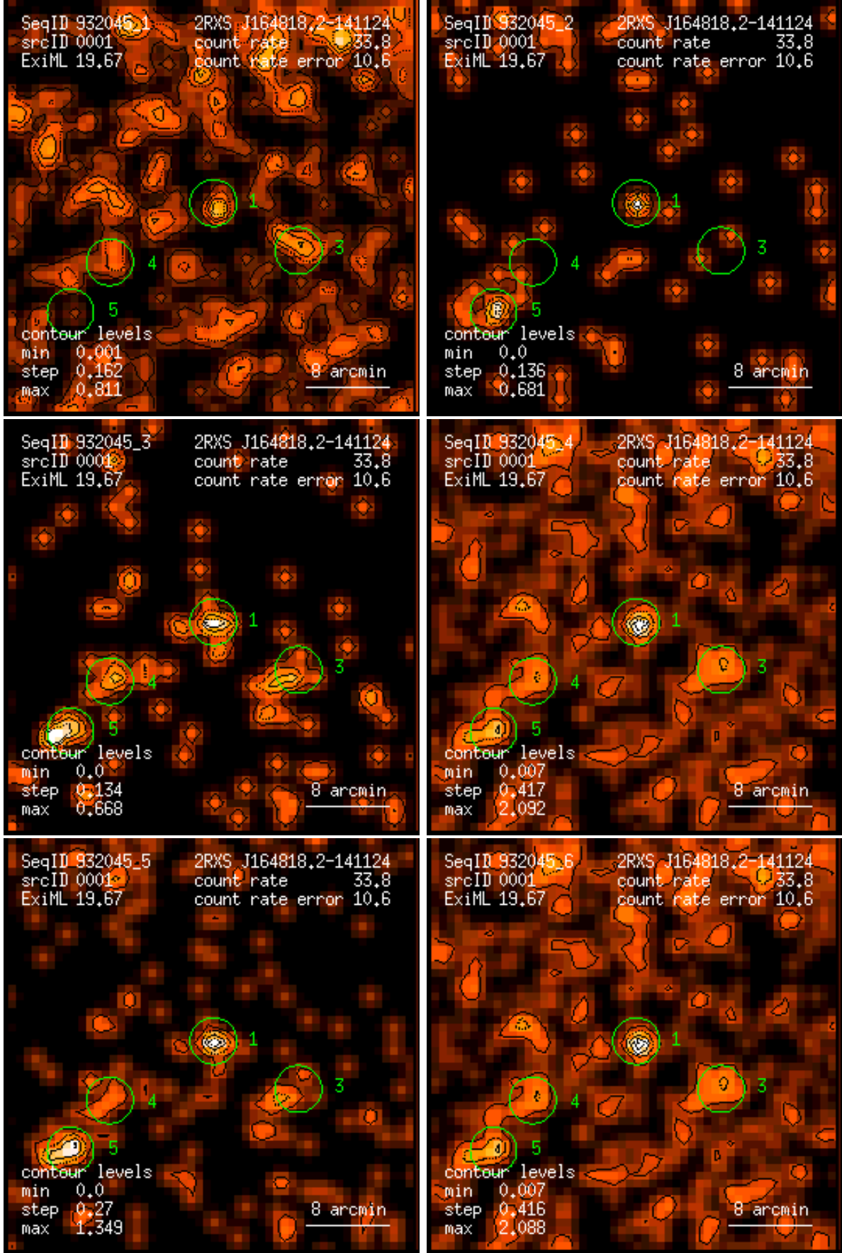
Figure 1: RASS 932045: detection 0001: band rate images, Gaussian filter: (1) PSPC channels 11 – 41, (2) 52 – 90, (3) 91 – 201, (4) 11 – 235, (5) 52 – 201, (6) 11 – 201. Broad band rates in counts/ks. Band rate contour levels in counts/ks/arcmin 2 .
