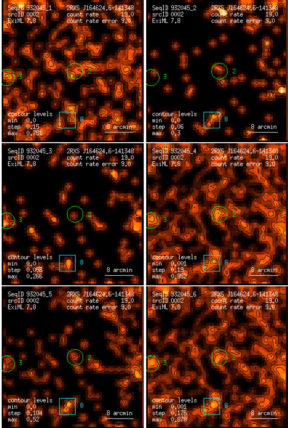
Figure 2: RASS 932045: detection 0002: band rate images, Gaussian filter: (1) PSPC channels 11 – 41, (2) 52 – 90, (3) 91 – 201, (4) 11 – 235, (5) 52 – 201, (6) 11 – 201. Broad band rates in counts/ks. Band rate contour levels in counts/ks/arcmin 2 .
