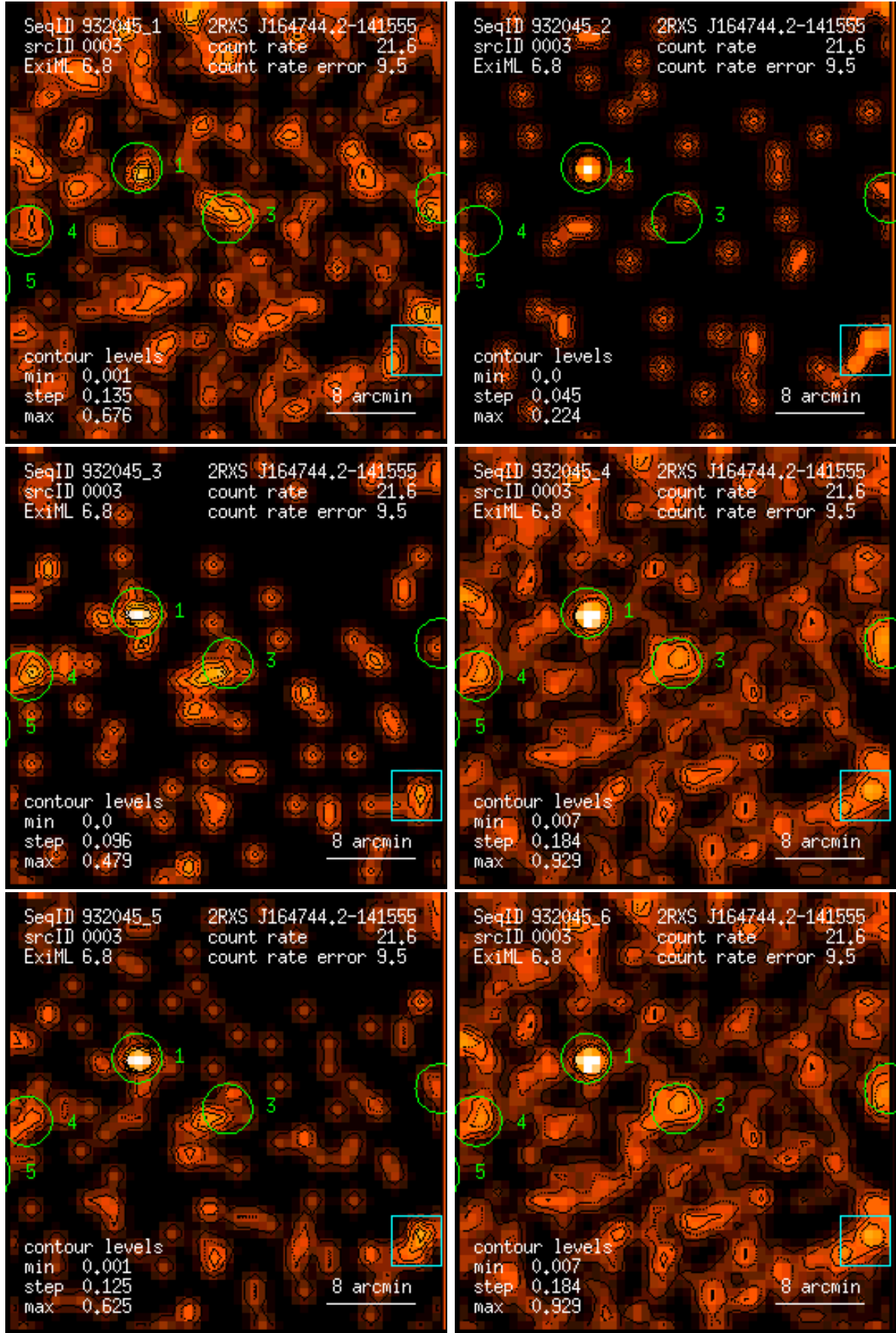
Figure 3: RASS 932045: detection 0003: band rate images, Gaussian filter: (1) PSPC channels 11 – 41, (2) 52 – 90, (3) 91 – 201, (4) 11 – 235, (5) 52 – 201, (6) 11 – 201. Broad band rates in counts/ks. Band rate contour levels in counts/ks/arcmin 2 .
