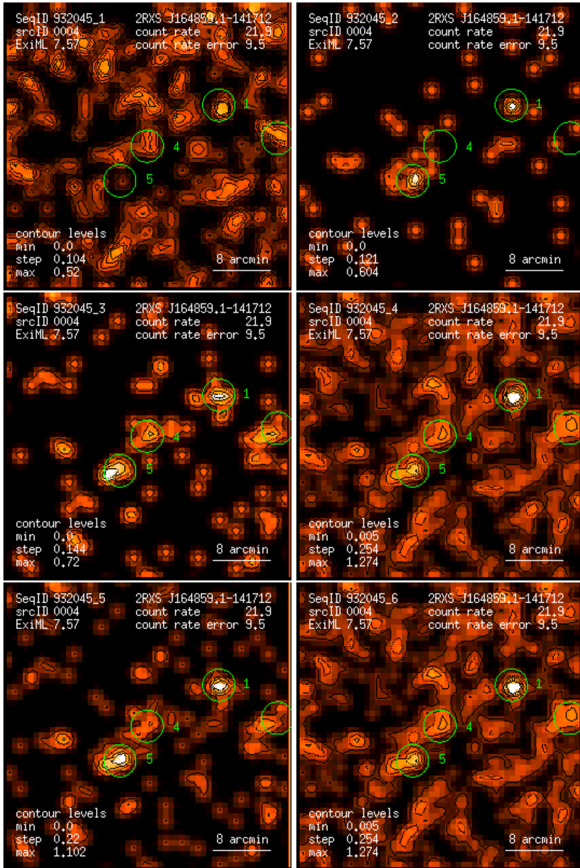
Figure 4: RASS 932045: detection 0004: band rate images, Gaussian filter: (1) PSPC channels 11 – 41, (2) 52 – 90, (3) 91 – 201, (4) 11 – 235, (5) 52 – 201, (6) 11 – 201. Broad band rates in counts/ks. Band rate contour levels in counts/ks/arcmin 2 .
