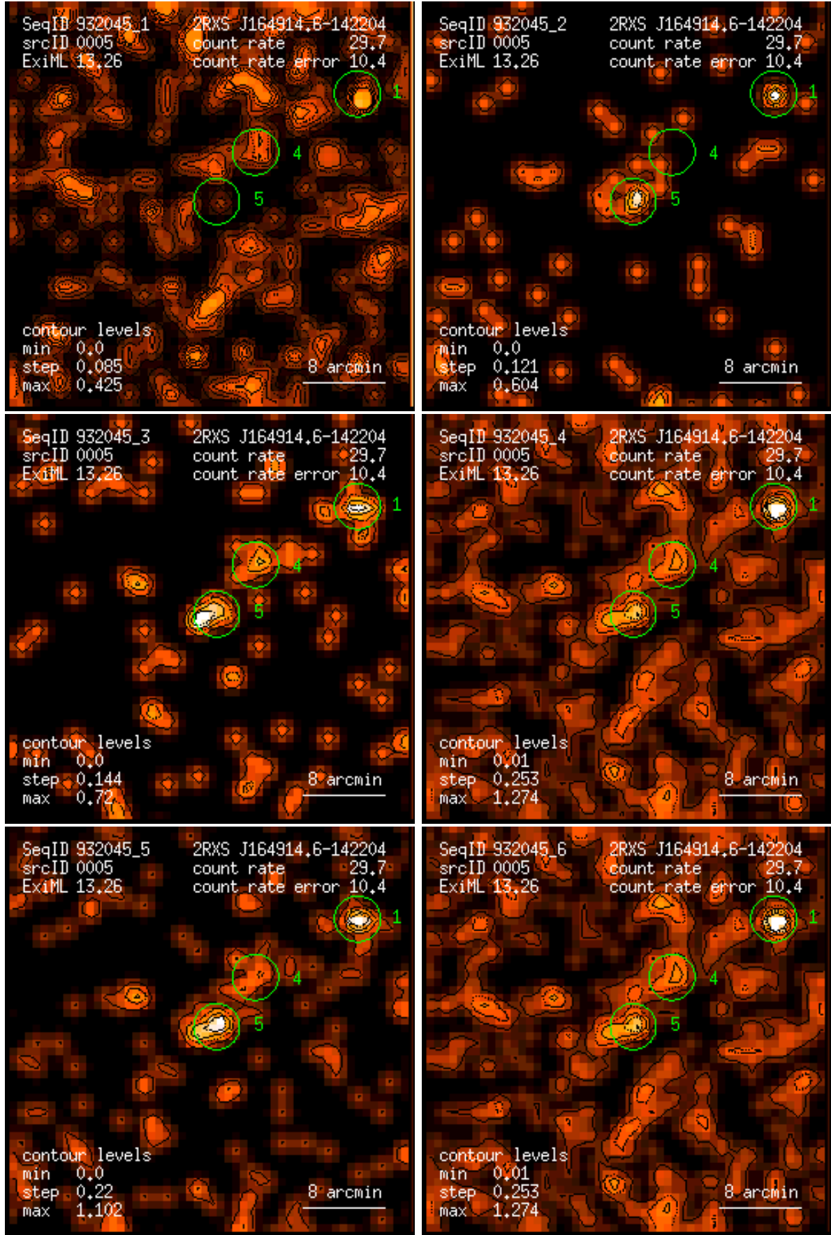
Figure 5: RASS 932045: detection 0005: band rate images, Gaussian filter: (1) PSPC channels 11 – 41, (2) 52 – 90, (3) 91 – 201, (4) 11 – 235, (5) 52 – 201, (6) 11 – 201. Broad band rates in counts/ks. Band rate contour levels in counts/ks/arcmin 2 .
