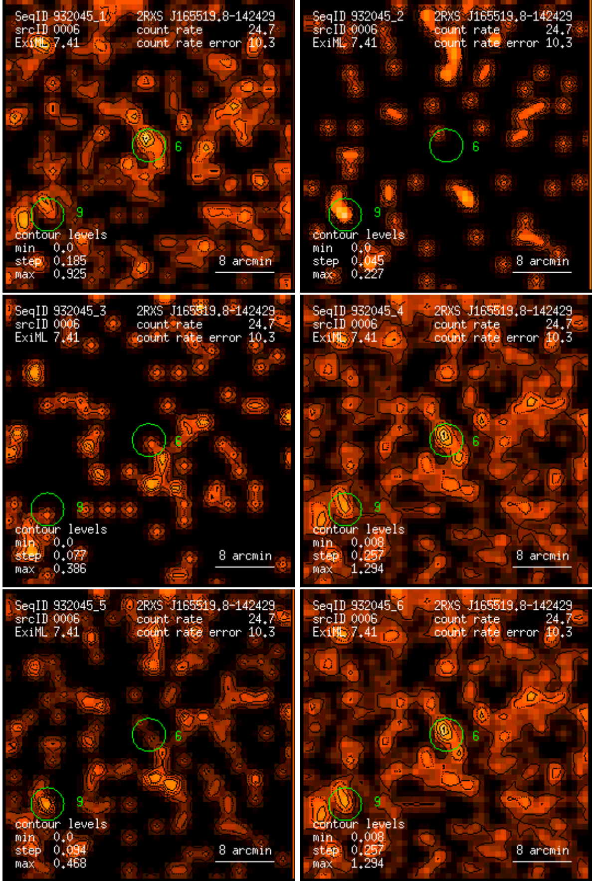
Figure 6: RASS 932045: detection 0006: band rate images, Gaussian filter: (1) PSPC channels 11 – 41, (2) 52 – 90, (3) 91 – 201, (4) 11 – 235, (5) 52 – 201, (6) 11 – 201. Broad band rates in counts/ks. Band rate contour levels in counts/ks/arcmin 2 .
