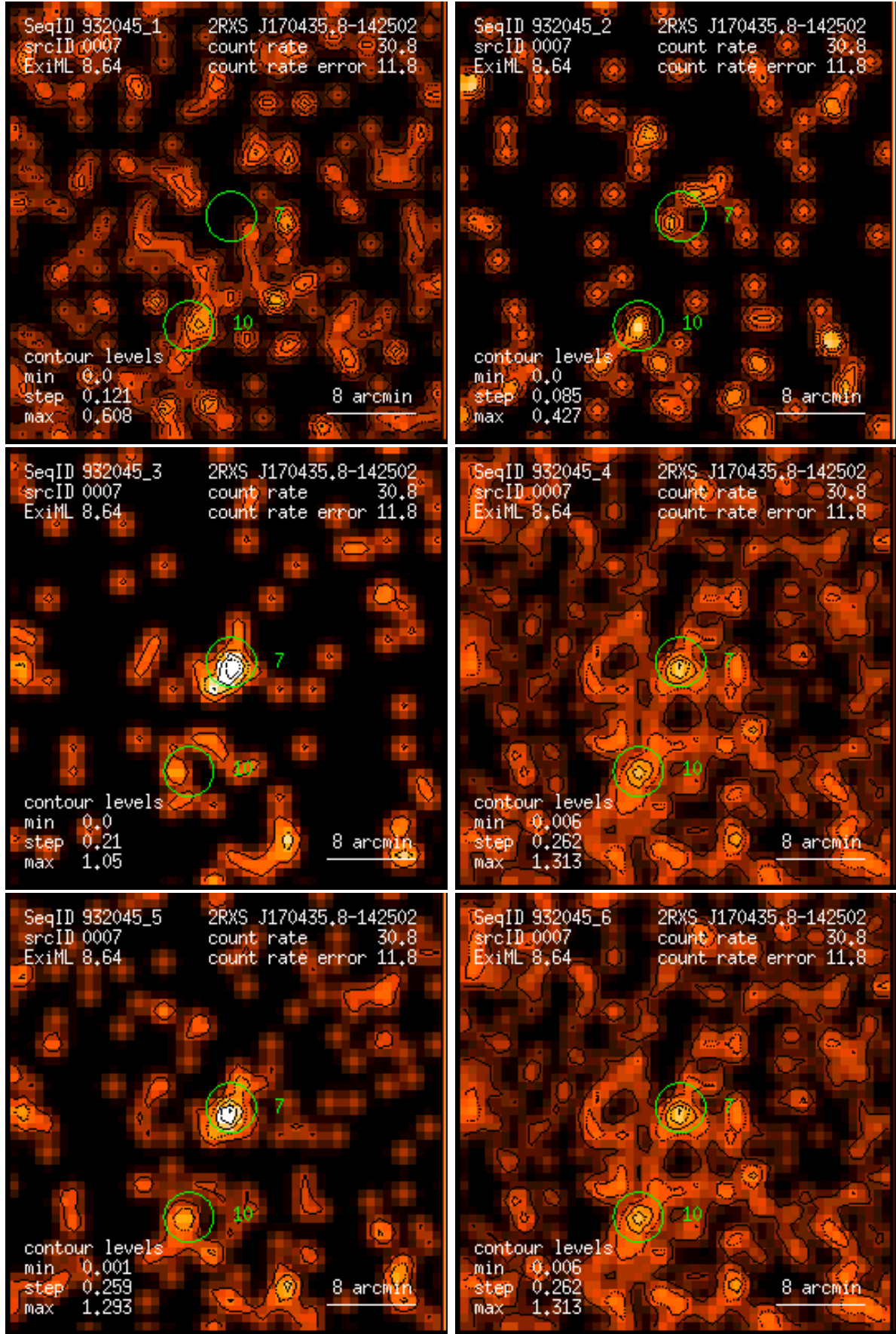
Figure 7: RASS 932045: detection 0007: band rate images, Gaussian filter: (1) PSPC channels 11 – 41, (2) 52 – 90, (3) 91 – 201, (4) 11 – 235, (5) 52 – 201, (6) 11 – 201. Broad band rates in counts/ks. Band rate contour levels in counts/ks/arcmin 2 .
