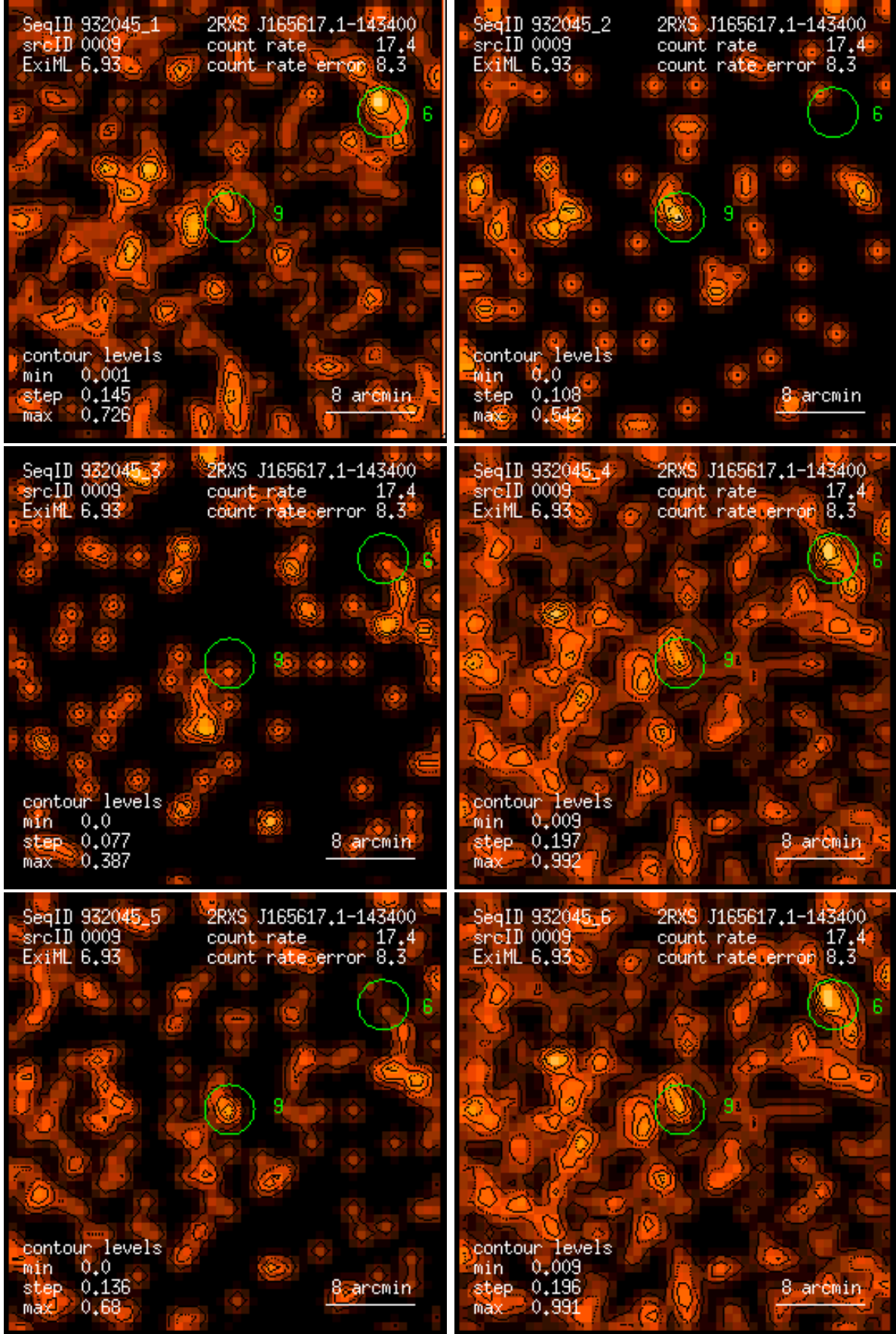
Figure 9: RASS 932045: detection 0009: band rate images, Gaussian filter: (1) PSPC channels 11 – 41, (2) 52 – 90, (3) 91 – 201, (4) 11 – 235, (5) 52 – 201, (6) 11 – 201. Broad band rates in counts/ks. Band rate contour levels in counts/ks/arcmin 2 .
