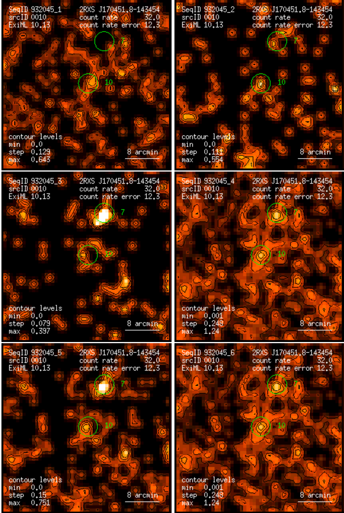
Figure 10: RASS 932045: detection 0010: band rate images, Gaussian filter: (1) PSPC channels 11 – 41, (2) 52 – 90, (3) 91 – 201, (4) 11 – 235, (5) 52 – 201, (6) 11 – 201. Broad band rates in counts/ks. Band rate contour levels in counts/ks/arcmin 2 .
