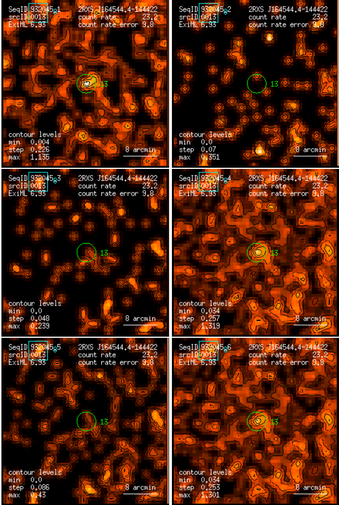
Figure 13: RASS 932045: detection 0013: band rate images, Gaussian filter: (1) PSPC channels 11 – 41, (2) 52 – 90, (3) 91 – 201, (4) 11 – 235, (5) 52 – 201, (6) 11 – 201. Broad band rates in counts/ks. Band rate contour levels in counts/ks/arcmin 2 .
