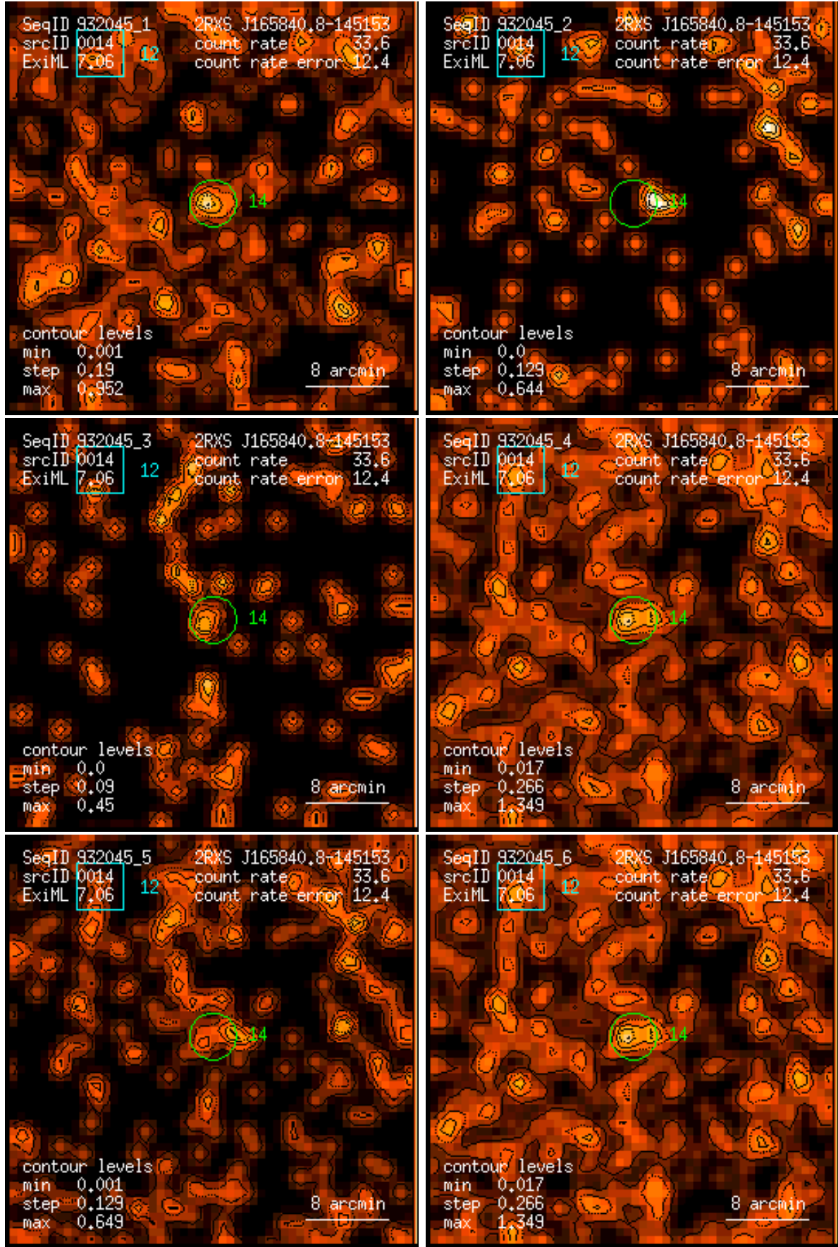
Figure 14: RASS 932045: detection 0014: band rate images, Gaussian filter: (1) PSPC channels 11 – 41, (2) 52 – 90, (3) 91 – 201, (4) 11 – 235, (5) 52 – 201, (6) 11 – 201. Broad band rates in counts/ks. Band rate contour levels in counts/ks/arcmin 2 .
