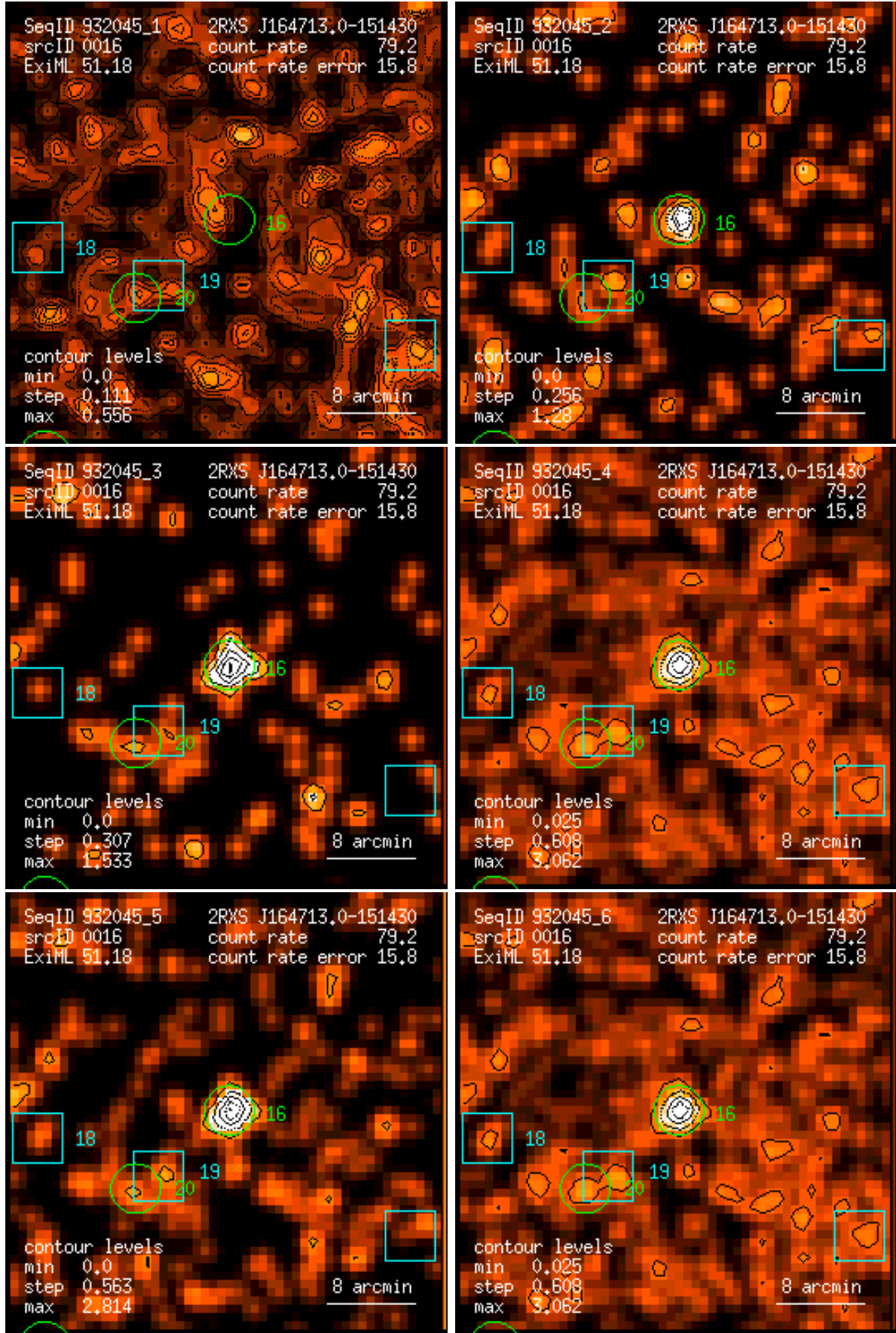
Figure 16: RASS 932045: detection 0016: band rate images, Gaussian filter: (1) PSPC channels 11 – 41, (2) 52 – 90, (3) 91 – 201, (4) 11 – 235, (5) 52 – 201, (6) 11 – 201. Broad band rates in counts/ks. Band rate contour levels in counts/ks/arcmin 2 .
