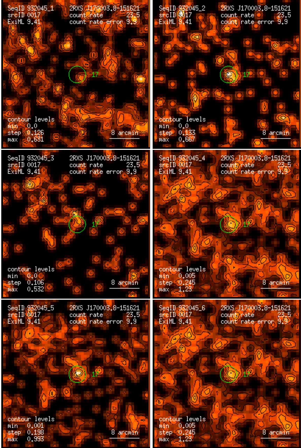
Figure 17: RASS 932045: detection 0017: band rate images, Gaussian filter: (1) PSPC channels 11 – 41, (2) 52 – 90, (3) 91 – 201, (4) 11 – 235, (5) 52 – 201, (6) 11 – 201. Broad band rates in counts/ks. Band rate contour levels in counts/ks/arcmin 2 .
