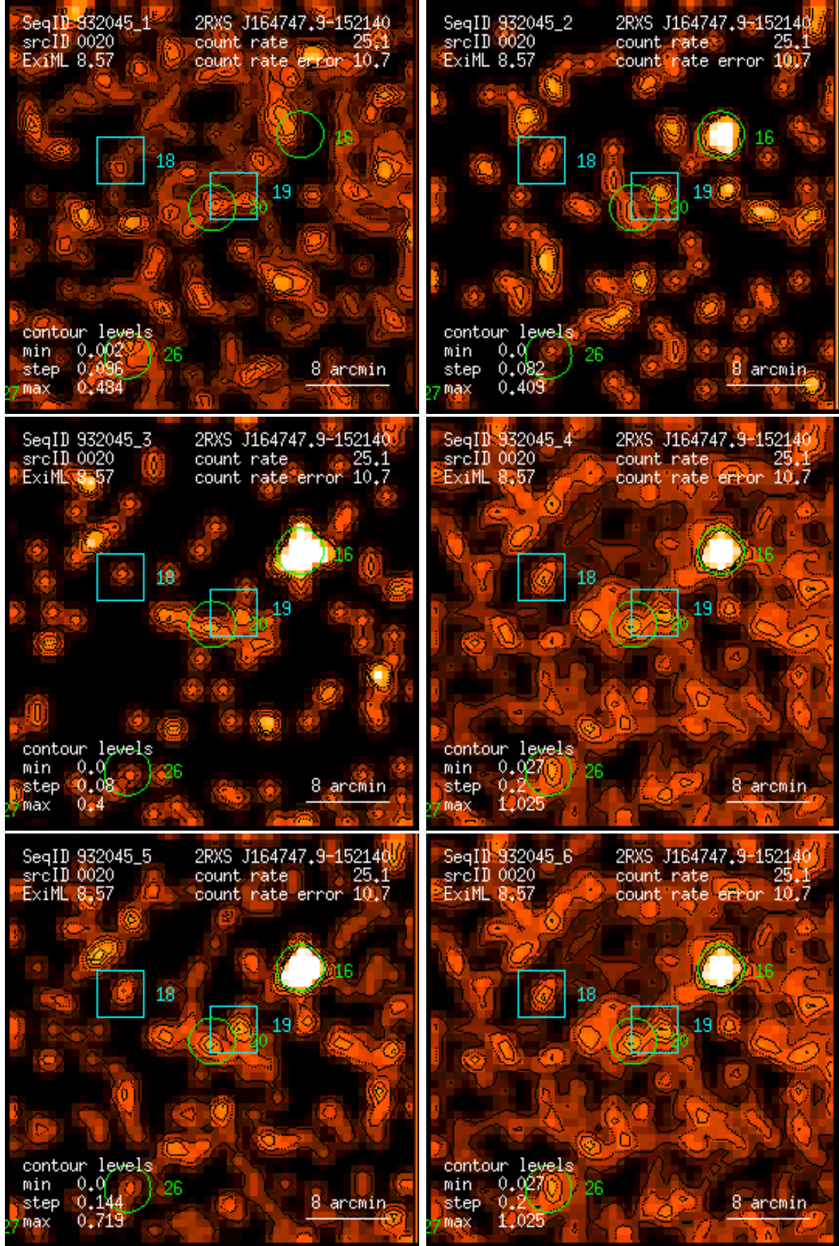
Figure 20: RASS 932045: detection 0020: band rate images, Gaussian filter: (1) PSPC channels 11 – 41, (2) 52 – 90, (3) 91 – 201, (4) 11 – 235, (5) 52 – 201, (6) 11 – 201. Broad band rates in counts/ks. Band rate contour levels in counts/ks/arcmin 2 .
