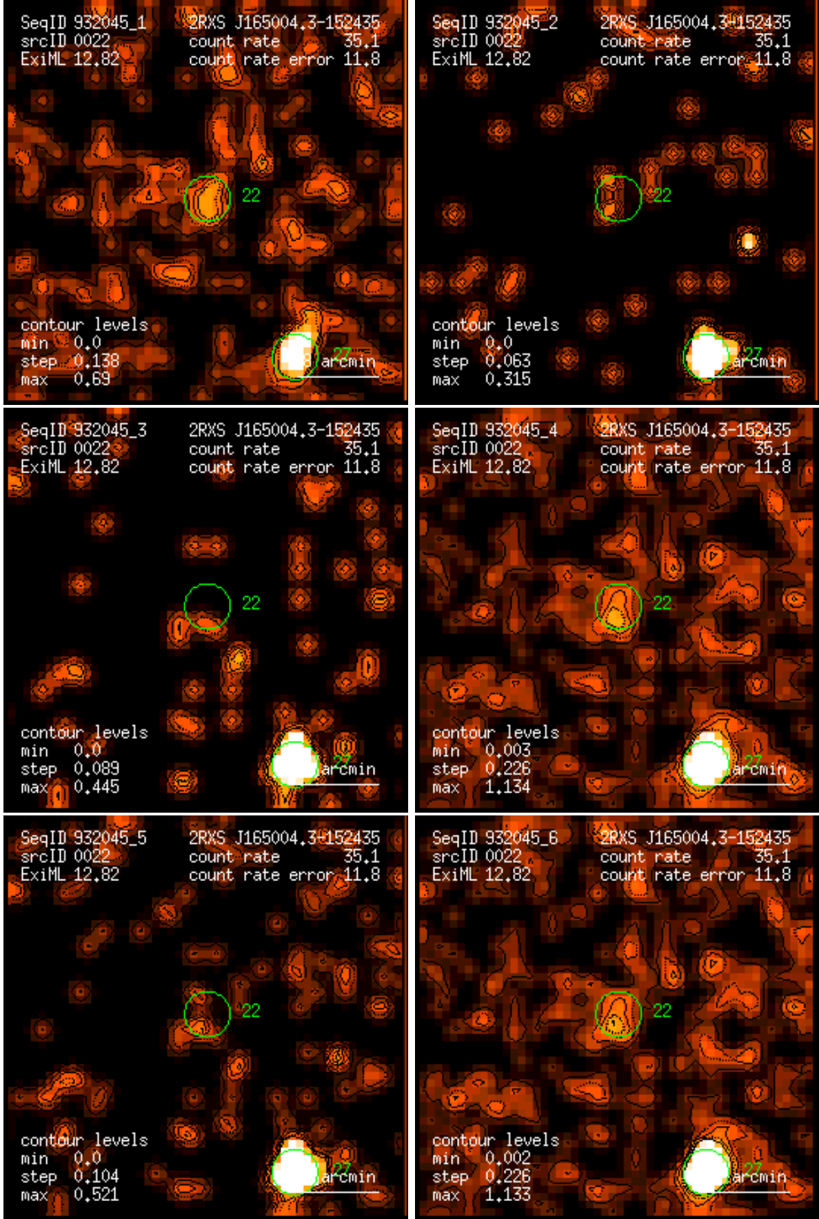
Figure 22: RASS 932045: detection 0022: band rate images, Gaussian filter: (1) PSPC channels 11 – 41, (2) 52 – 90, (3) 91 – 201, (4) 11 – 235, (5) 52 – 201, (6) 11 – 201. Broad band rates in counts/ks. Band rate contour levels in counts/ks/arcmin 2 .
