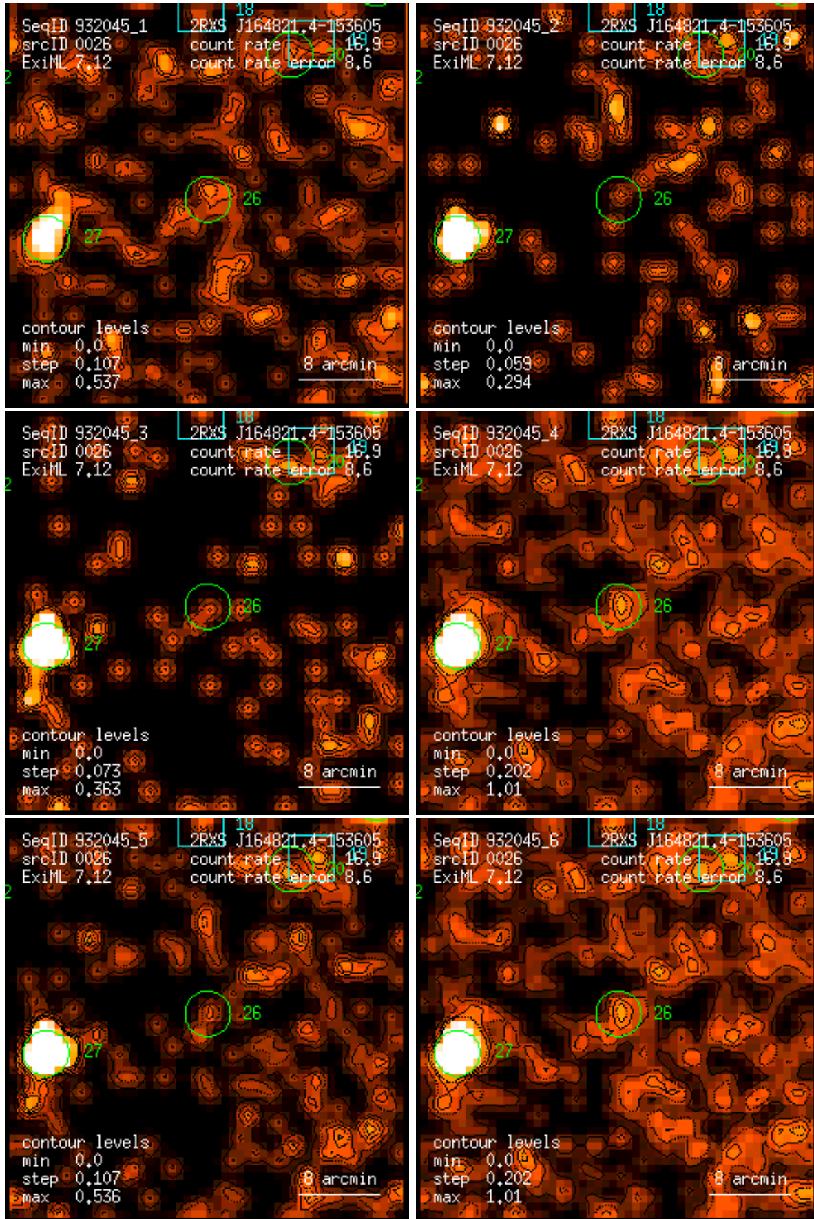
Figure 26: RASS 932045: detection 0026: band rate images, Gaussian filter: (1) PSPC channels 11 – 41, (2) 52 – 90, (3) 91 – 201, (4) 11 – 235, (5) 52 – 201, (6) 11 – 201. Broad band rates in counts/ks. Band rate contour levels in counts/ks/arcmin 2 .
