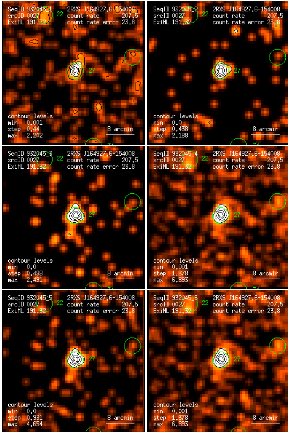
Figure 27: RASS 932045: detection 0027: band rate images, Gaussian filter: (1) PSPC channels 11 – 41, (2) 52 – 90, (3) 91 – 201, (4) 11 – 235, (5) 52 – 201, (6) 11 – 201. Broad band rates in counts/ks. Band rate contour levels in counts/ks/arcmin 2 .
