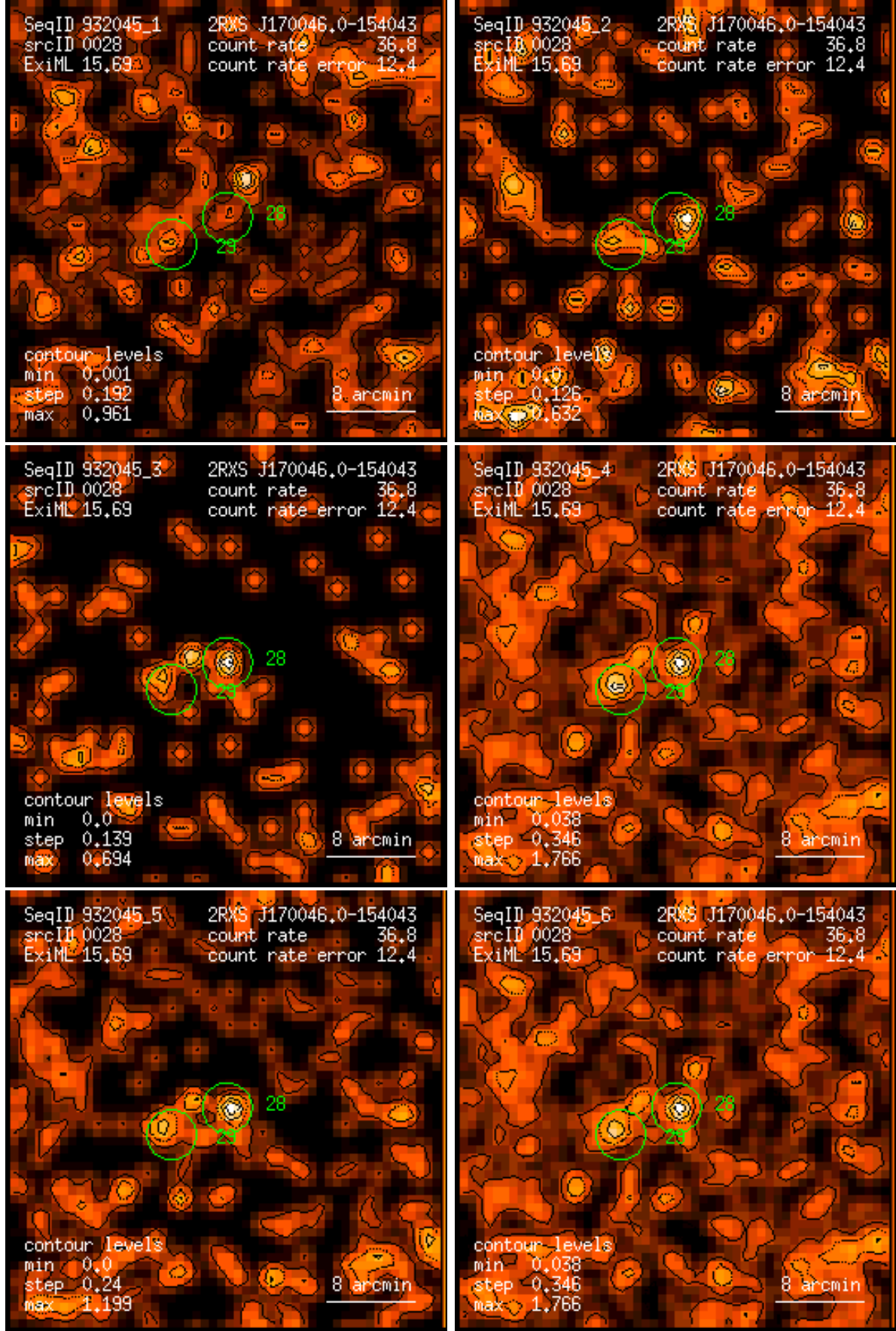
Figure 28: RASS 932045: detection 0028: band rate images, Gaussian filter: (1) PSPC channels 11 – 41, (2) 52 – 90, (3) 91 – 201, (4) 11 – 235, (5) 52 – 201, (6) 11 – 201. Broad band rates in counts/ks. Band rate contour levels in counts/ks/arcmin 2 .
