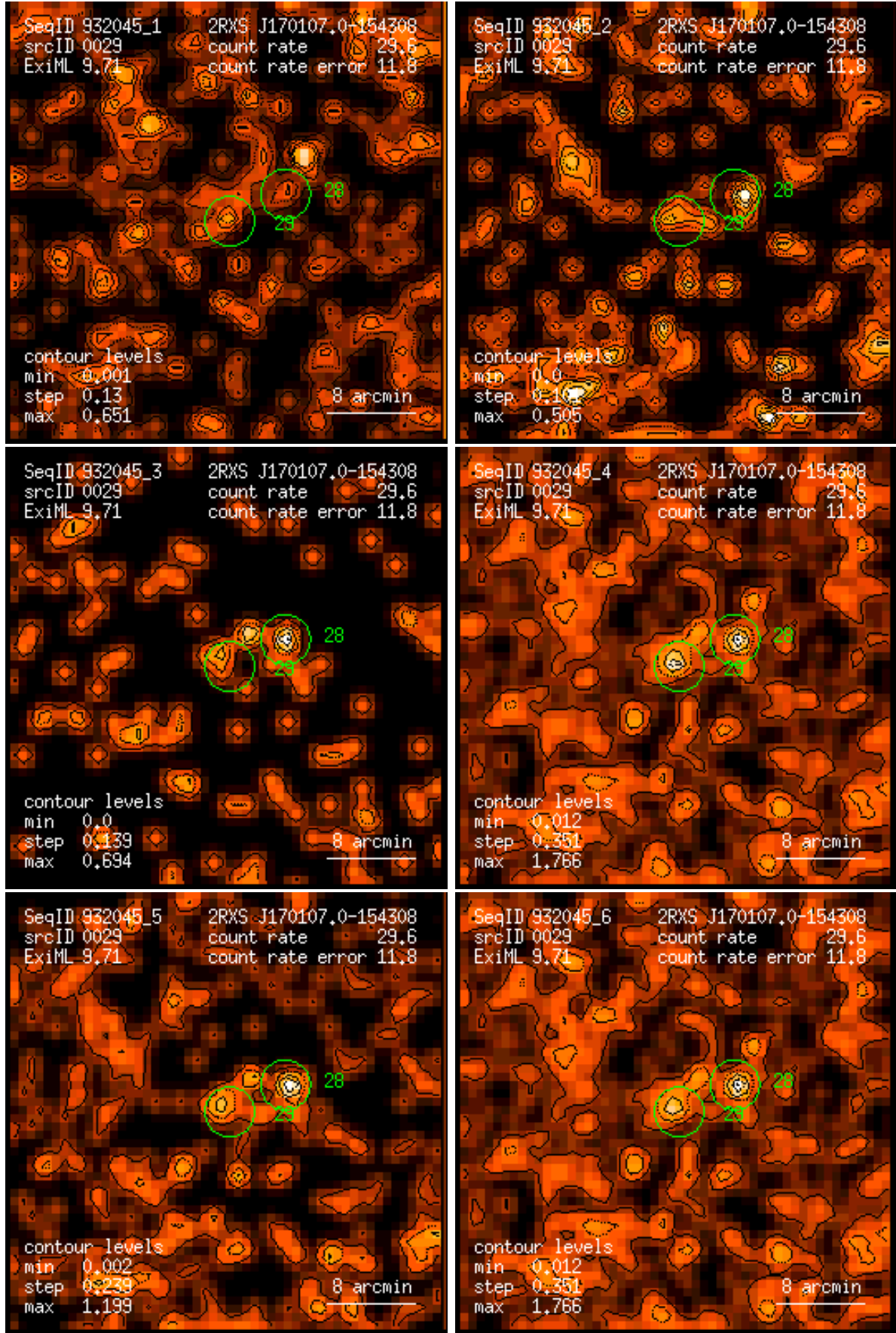
Figure 29: RASS 932045: detection 0029: band rate images, Gaussian filter: (1) PSPC channels 11 – 41, (2) 52 – 90, (3) 91 – 201, (4) 11 – 235, (5) 52 – 201, (6) 11 – 201. Broad band rates in counts/ks. Band rate contour levels in counts/ks/arcmin 2 .
