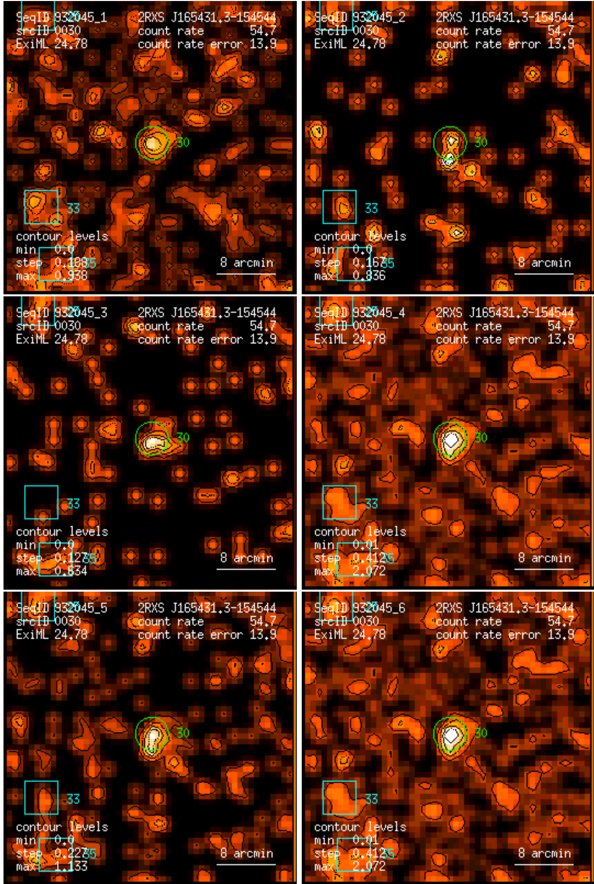
Figure 30: RASS 932045: detection 0030: band rate images, Gaussian filter: (1) PSPC channels 11 – 41, (2) 52 – 90, (3) 91 – 201, (4) 11 – 235, (5) 52 – 201, (6) 11 – 201. Broad band rates in counts/ks. Band rate contour levels in counts/ks/arcmin 2 .
