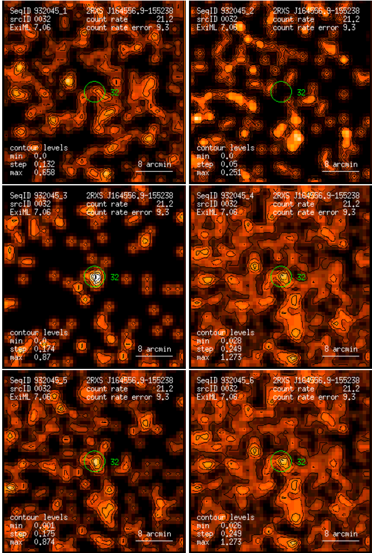
Figure 32: RASS 932045: detection 0032: band rate images, Gaussian filter: (1) PSPC channels 11 – 41, (2) 52 – 90, (3) 91 – 201, (4) 11 – 235, (5) 52 – 201, (6) 11 – 201. Broad band rates in counts/ks. Band rate contour levels in counts/ks/arcmin 2 .
