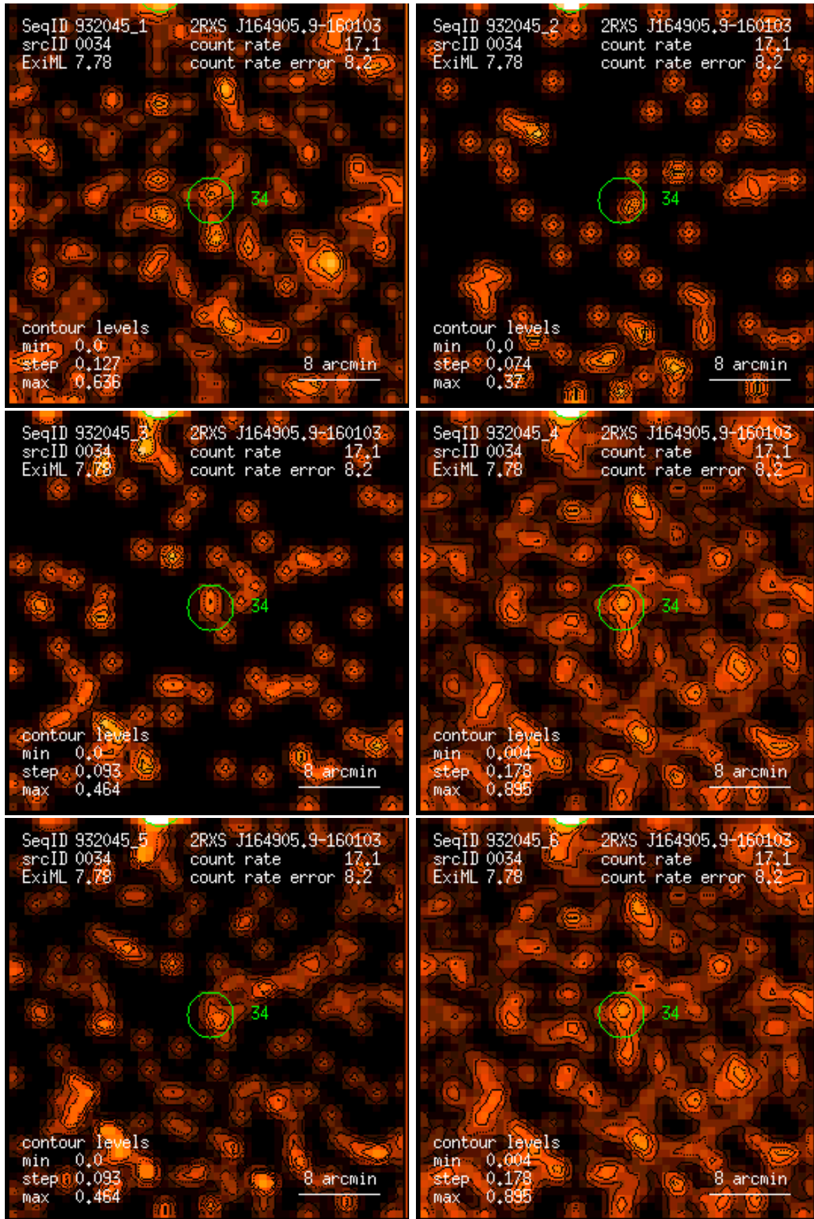
Figure 34: RASS 932045: detection 0034: band rate images, Gaussian filter: (1) PSPC channels 11 – 41, (2) 52 – 90, (3) 91 – 201, (4) 11 – 235, (5) 52 – 201, (6) 11 – 201. Broad band rates in counts/ks. Band rate contour levels in counts/ks/arcmin 2 .
