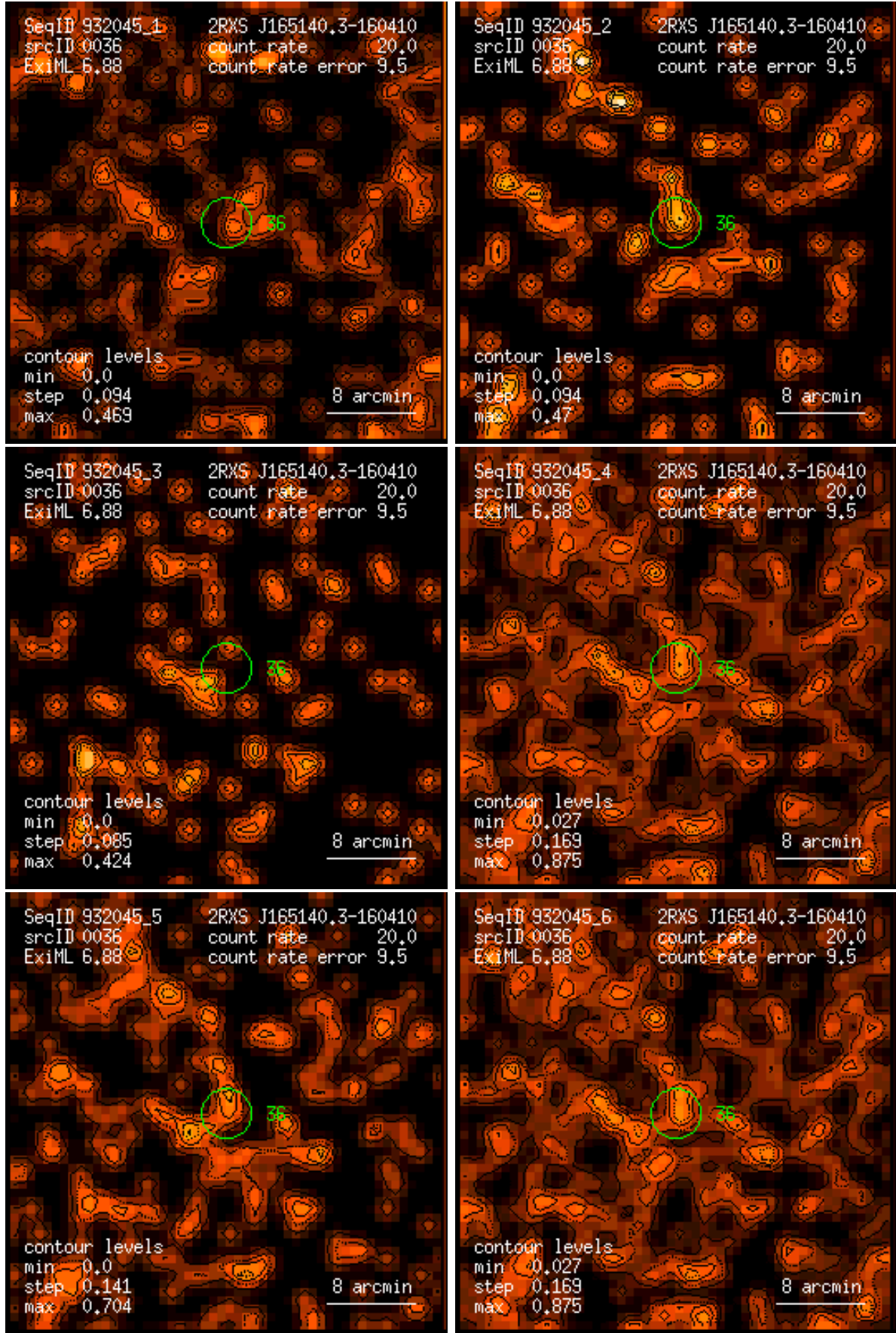
Figure 36: RASS 932045: detection 0036: band rate images, Gaussian filter: (1) PSPC channels 11 – 41, (2) 52 – 90, (3) 91 – 201, (4) 11 – 235, (5) 52 – 201, (6) 11 – 201. Broad band rates in counts/ks. Band rate contour levels in counts/ks/arcmin 2 .
