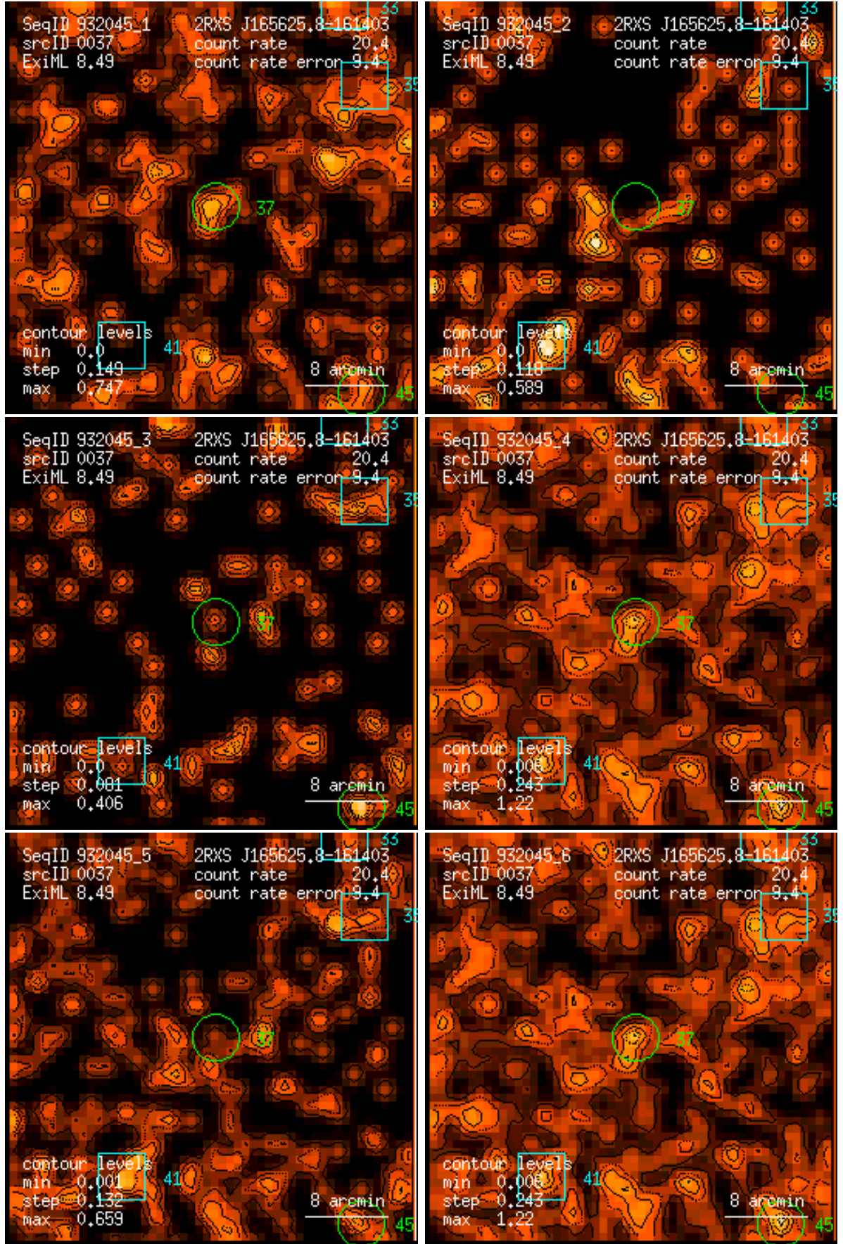
Figure 37: RASS 932045: detection 0037: band rate images, Gaussian filter: (1) PSPC channels 11 – 41, (2) 52 – 90, (3) 91 – 201, (4) 11 – 235, (5) 52 – 201, (6) 11 – 201. Broad band rates in counts/ks. Band rate contour levels in counts/ks/arcmin 2 .
