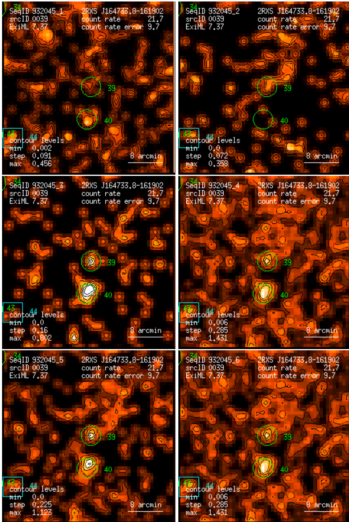
Figure 39: RASS 932045: detection 0039: band rate images, Gaussian filter: (1) PSPC channels 11 – 41, (2) 52 – 90, (3) 91 – 201, (4) 11 – 235, (5) 52 – 201, (6) 11 – 201. Broad band rates in counts/ks. Band rate contour levels in counts/ks/arcmin 2 .
