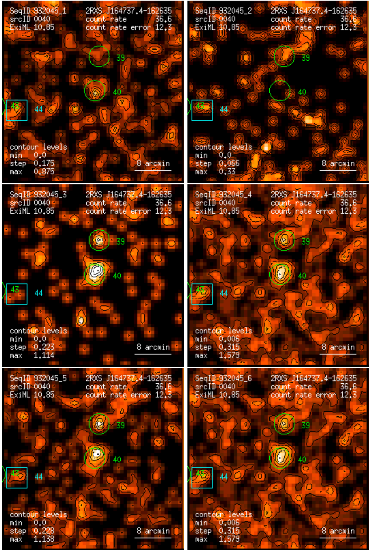
Figure 40: RASS 932045: detection 0040: band rate images, Gaussian filter: (1) PSPC channels 11 – 41, (2) 52 – 90, (3) 91 – 201, (4) 11 – 235, (5) 52 – 201, (6) 11 – 201. Broad band rates in counts/ks. Band rate contour levels in counts/ks/arcmin 2 .
