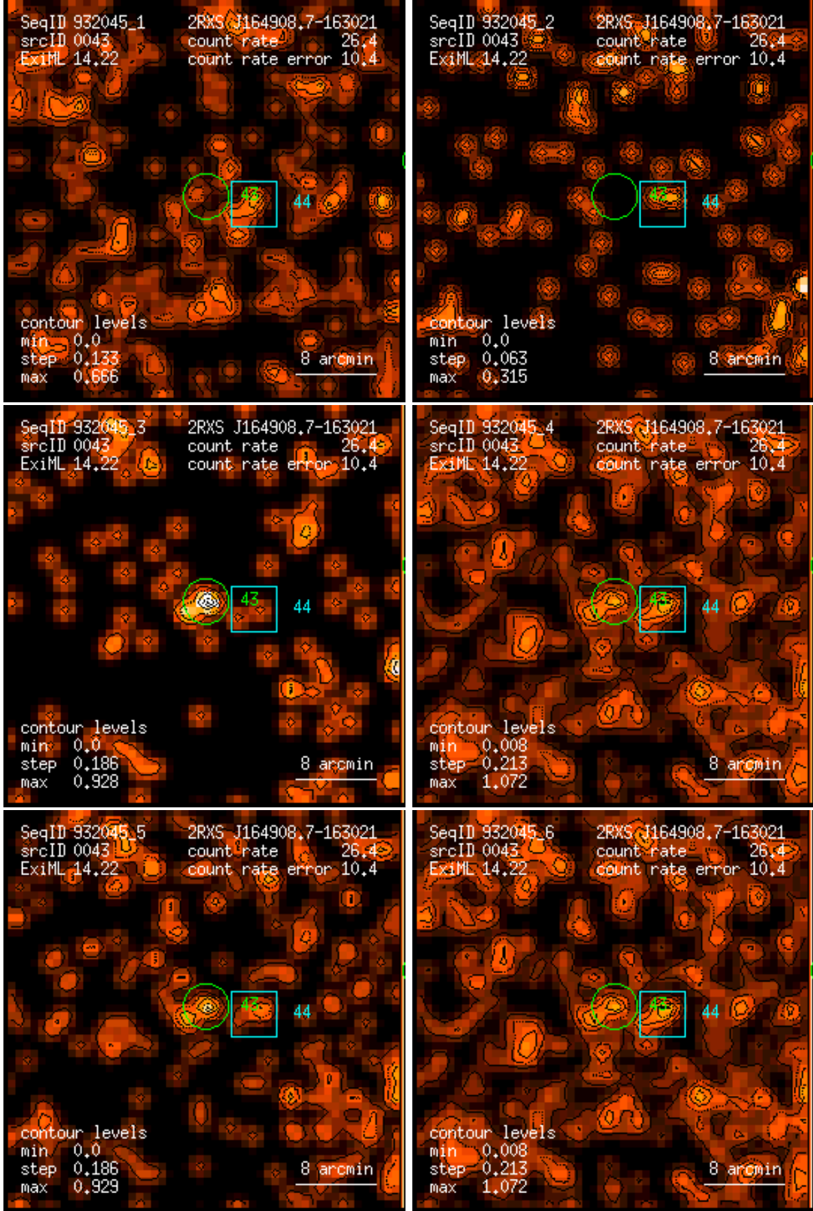
Figure 43: RASS 932045: detection 0043: band rate images, Gaussian filter: (1) PSPC channels 11 – 41, (2) 52 – 90, (3) 91 – 201, (4) 11 – 235, (5) 52 – 201, (6) 11 – 201. Broad band rates in counts/ks. Band rate contour levels in counts/ks/arcmin 2 .
